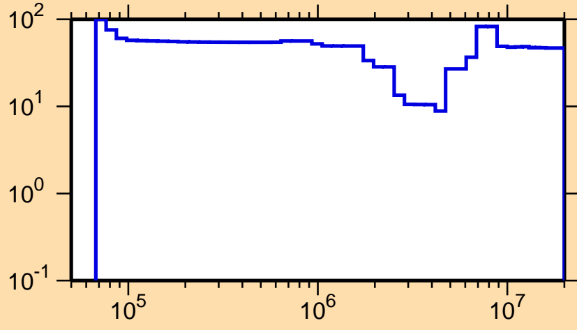
\Delta\sigma/\sigma vs. E for ^{183}\text{Hf}(n,\text{inel.})
