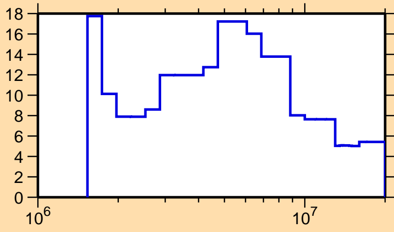
\Delta\sigma/\sigma vs. E for ^{183}\text{Hf}(n, tot.)
