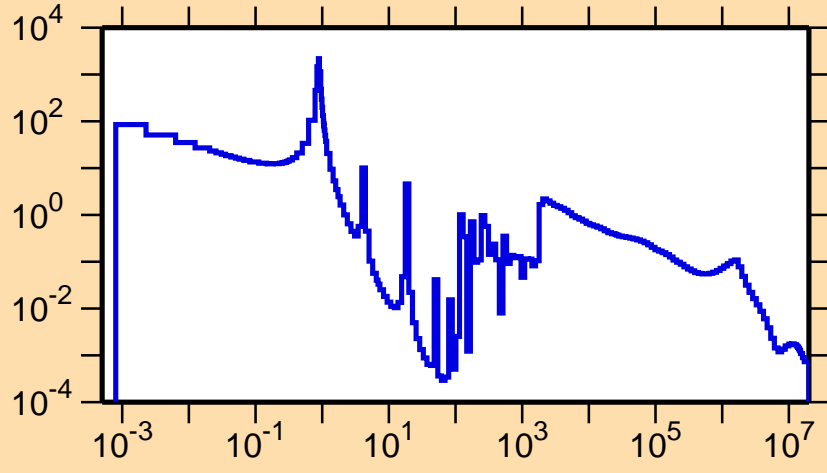
\sigma vs. E for ^{183}\text{Hf}(n,\gamma)
