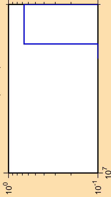
\Delta\sigma/\sigma vs. E for ^{183}\text{Hf}(n,3n\alpha)
