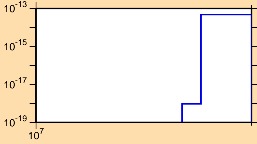
\sigma vs. E for ^{183}\text{Hf}(n,\text{He3})
