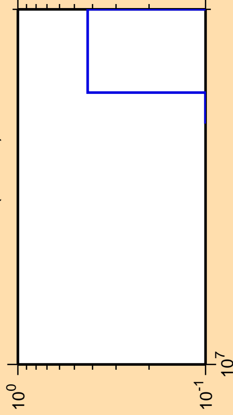
\Delta\sigma/\sigma vs. E for ^{183}\text{Hf}(n,\text{He3})
