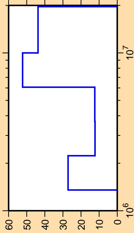
\Delta\sigma/\sigma vs. E for ^{183}\text{Hf}(n,n\text{cont.})
