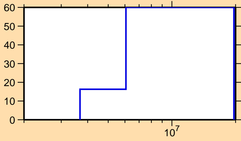
\Delta\sigma/\sigma vs. E for ^{183}\text{Hf}(n,p)
