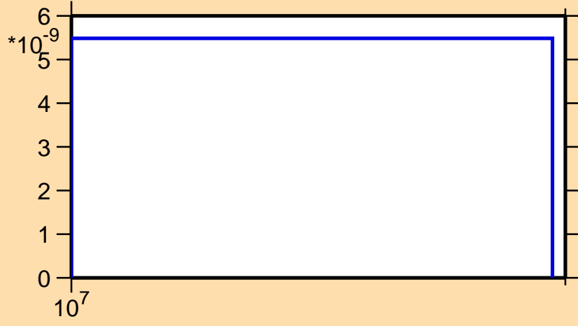
\sigma vs. E for ^{183}\text{Hf}(n,nt)
