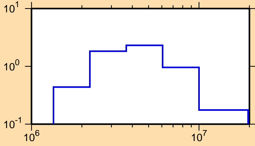
\sigma vs. E for ^{183}\text{Hf}(n,n\text{cont.})
