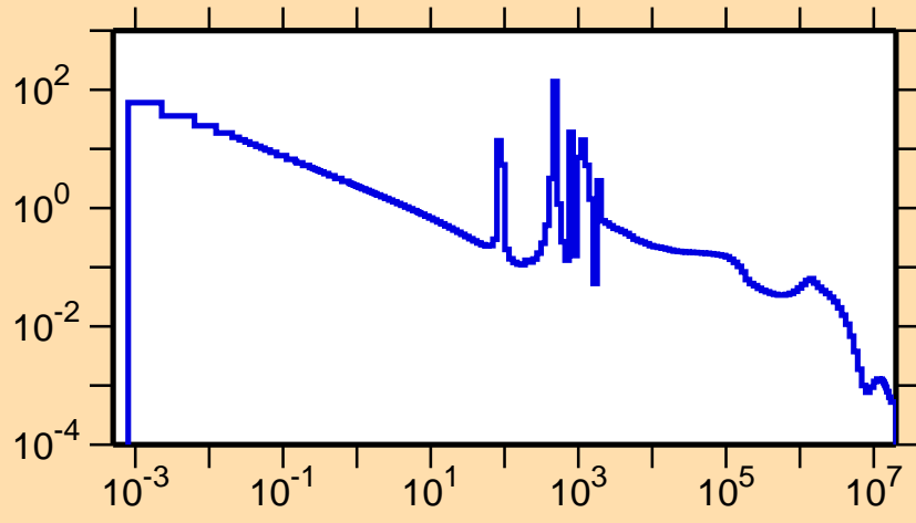
\sigma vs. E for ^{184}\text{Hf}(n,\gamma)
