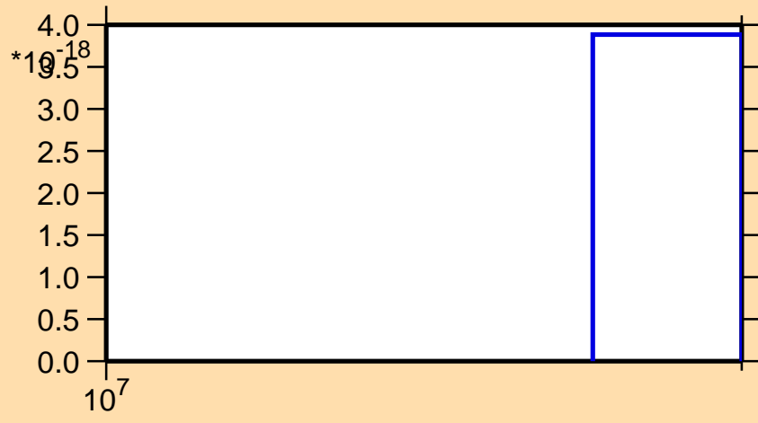
\sigma vs. E for ^{184}\text{Hf} (mt 11)
