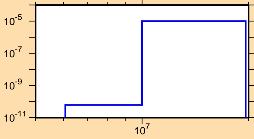
\sigma vs. E for ^{184}\text{Hf}(n,n\alpha)
