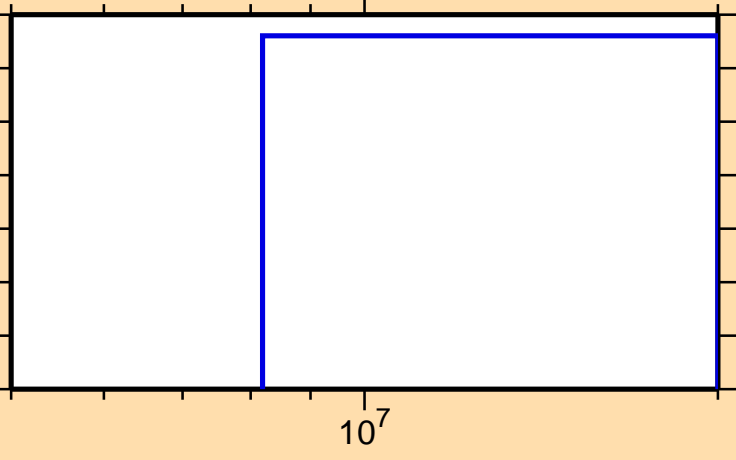
\sigma vs. E for ^{184}\text{Hf}(n,d)
