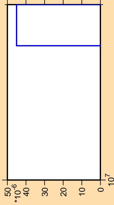
\Delta\sigma/\sigma vs. E for ^{184}\text{Hf} (mt 42)
