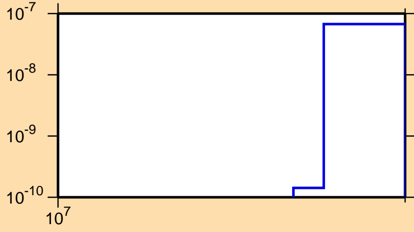
\sigma vs. E for ^{184}\text{Hf}(n,2np)
