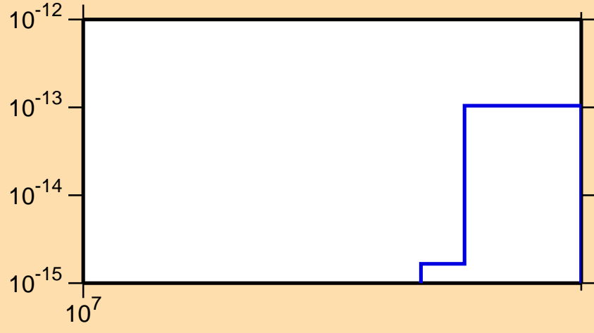
\sigma vs. E for ^{184}\text{Hf}(n,\text{He3})
