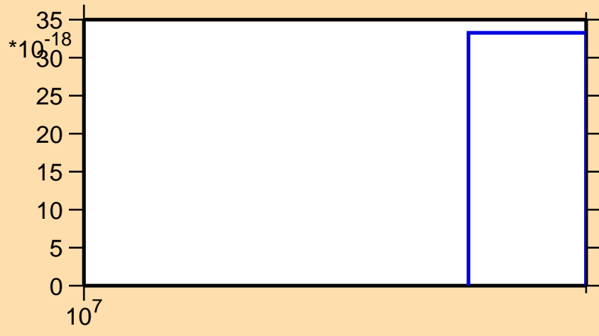
\sigma vs. E for ^{184}\text{Hf} (mt 42)
