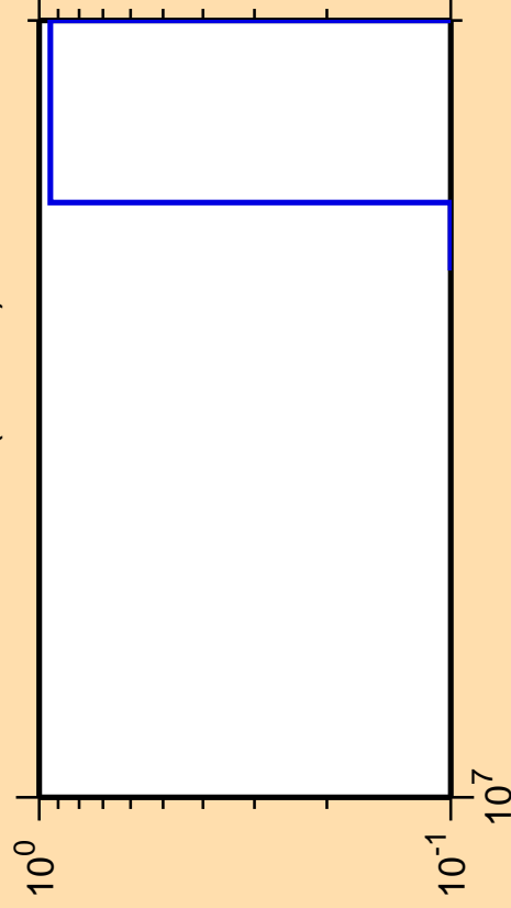
\Delta\sigma/\sigma vs. E for ^{184}\text{Hf}(n,\text{He3})
