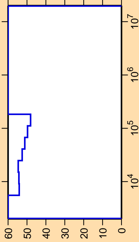
\Delta\sigma/\sigma vs. E for ^{184}\text{Hf}(n,n_3)
