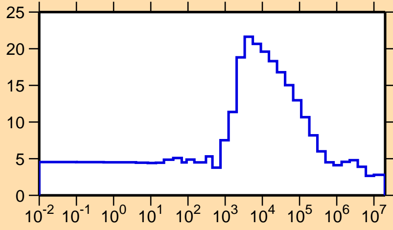
\sigma vs. E for ^{184}\text{Hf}(n,\text{el.})
