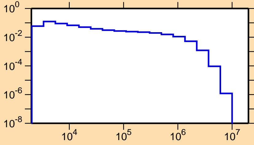
\sigma vs. E for ^{184}\text{Hf}(n,n_3)
