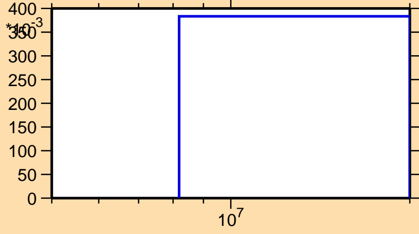
\sigma vs. E for ^{184}\text{Hf}(n,3n)
