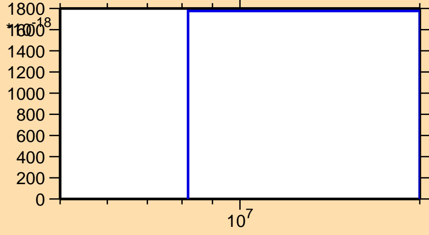
\sigma vs. E for ^{184}\text{Hf}(n,\text{He3})
