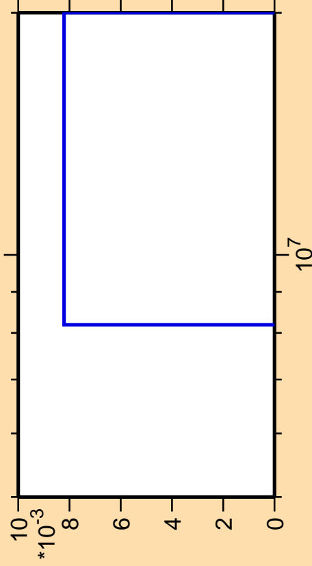
\Delta\sigma/\sigma vs. E for ^{184}\text{Hf}(n,\text{He3})
