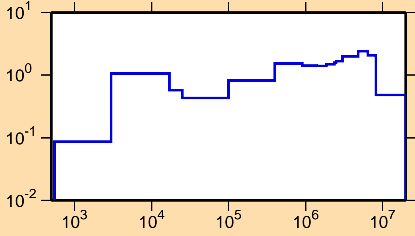
\sigma vs. E for ^{184}\text{Hf}(n,\text{inel.})
