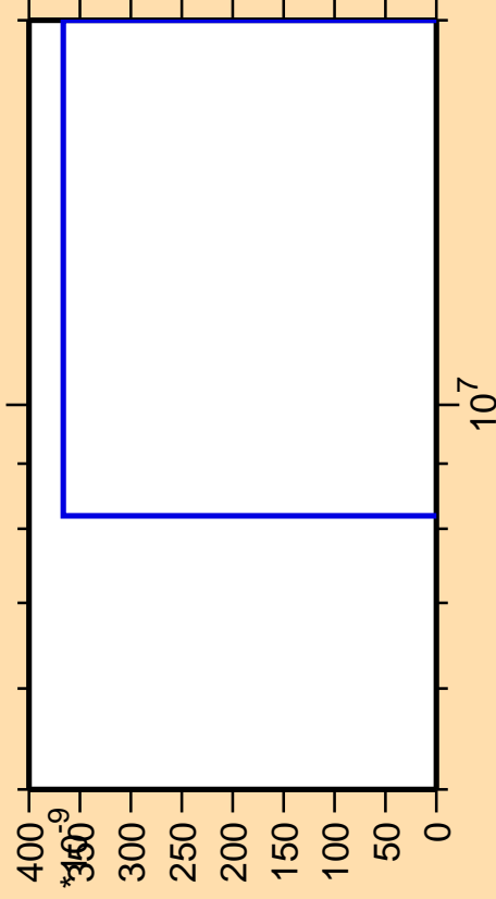
\Delta\sigma/\sigma vs. E for ^{184}\text{Hf}(\text{mt } 42)
