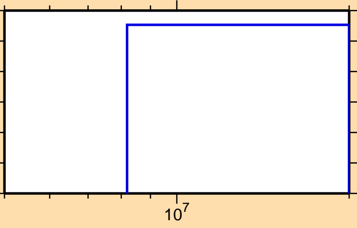
\sigma vs. E for ^{184}\text{Hf}(n,2np)
