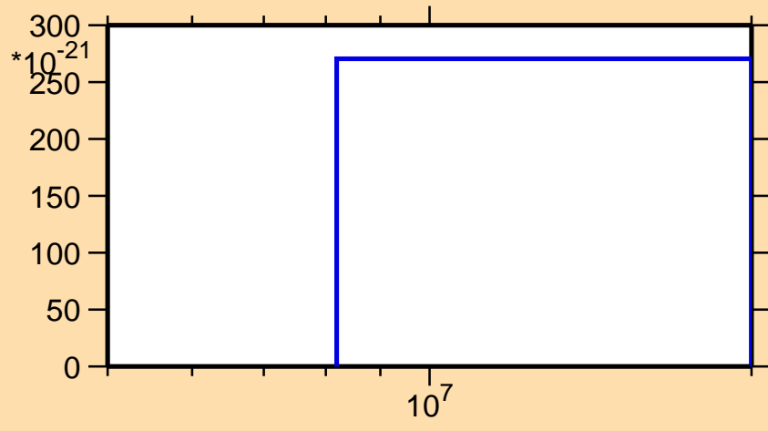
\sigma vs. E for ^{184}\text{Hf}(\text{mt } 42)
