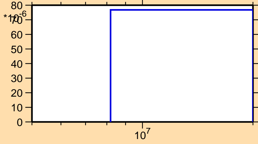
\sigma vs. E for ^{184}\text{Hf}(n,d)
