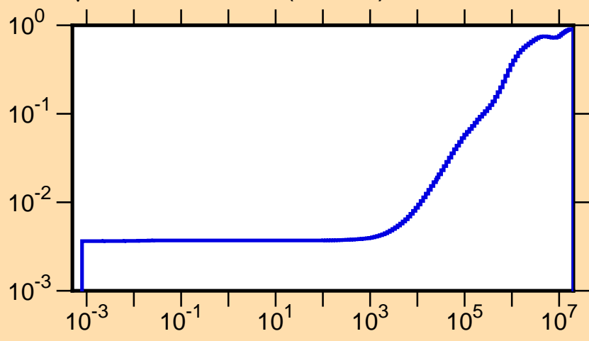
\mu vs. E for ^{185}\text{Hf}(\text{mt251})
