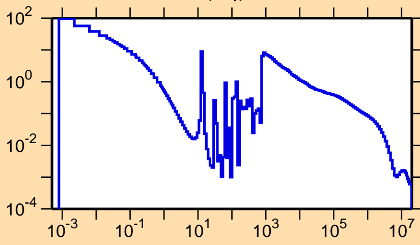
\sigma vs. E for ^{185}\text{Hf}(n,\gamma)
