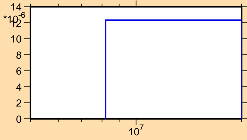
\sigma vs. E for ^{185}\text{Hf}(n,t)
