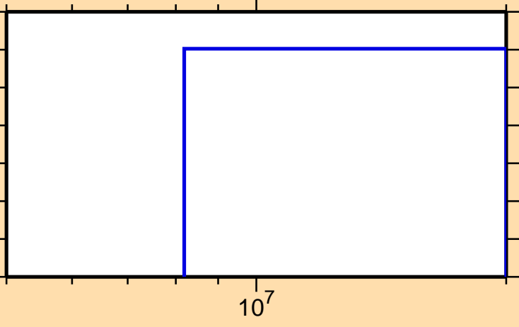
\sigma vs. E for ^{185}\text{Hf}(n,nt)
