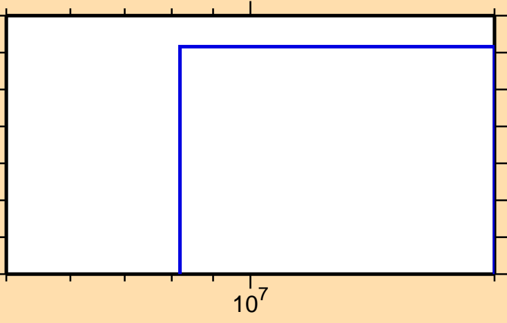
\sigma vs. E for ^{185}\text{Hf}(n,t)
