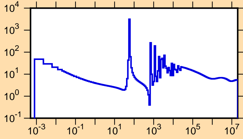
\sigma vs. E for ^{186}\text{Hf}(n,\text{tot.})
