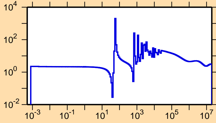
\sigma vs. E for ^{186}\text{Hf}(n,\text{el.})
