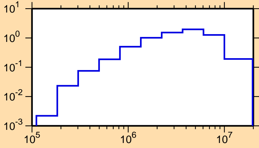
\sigma vs. E for ^{186}\text{Hf}(n,n\text{cont.})
