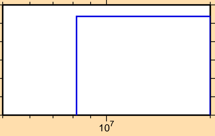
\sigma vs. E for ^{186}\text{Hf}(n,2n\alpha)
