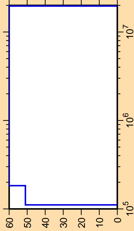
\Delta\sigma/\sigma vs. E for ^{187}\text{Hf}(n,\gamma)
