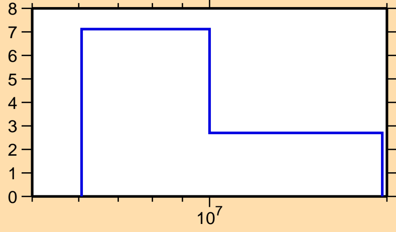
\Delta\sigma/\sigma vs. E for ^{187}\text{Hf}(n,\text{tot.})
