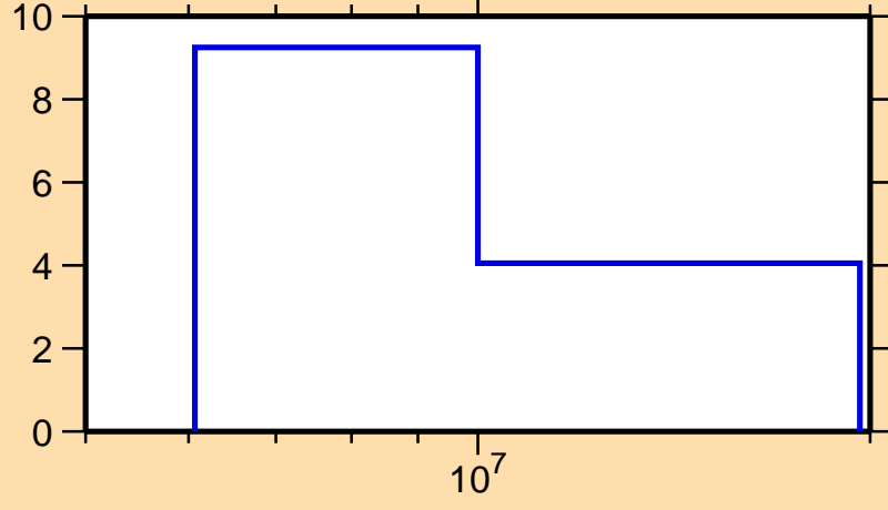
\Delta\sigma/\sigma vs. E for ^{188}\text{Hf}(n,\text{tot.})
