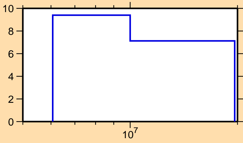
\Delta\sigma/\sigma vs. E for ^{188}\text{Hf}(n,\text{nonel.})
