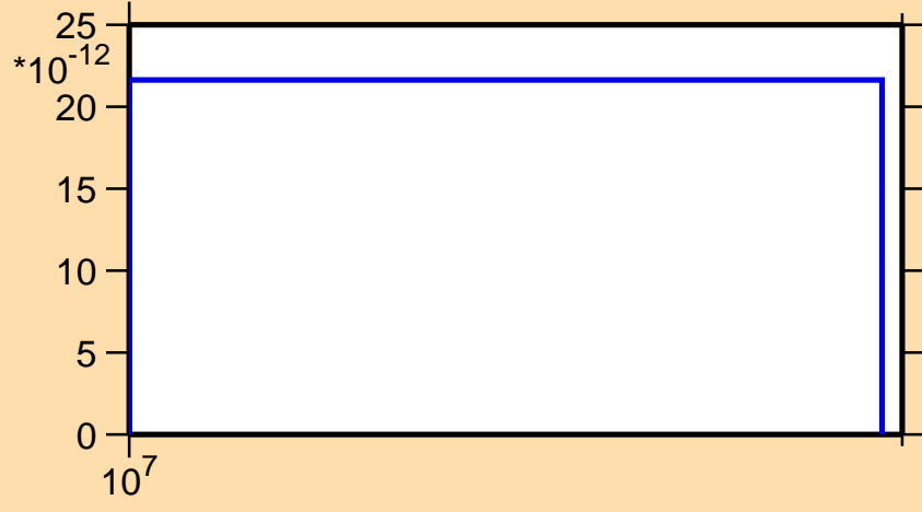
\sigma vs. E for ^{188}\text{Hf}(n,\text{nd})
