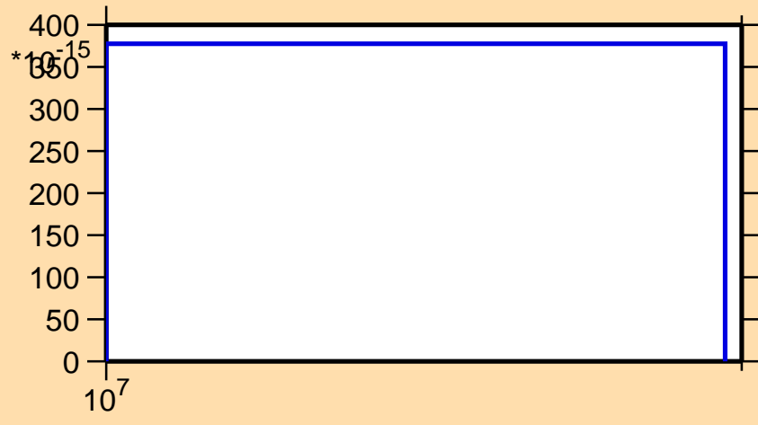
\sigma vs. E for ^{188}\text{Hf}(n,2np)
