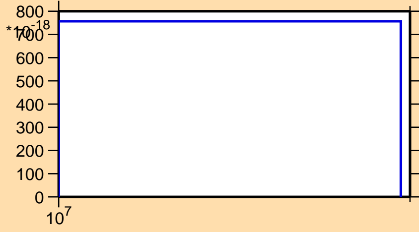
\sigma vs. E for ^{188}\text{Hf}(n,3n\alpha)
