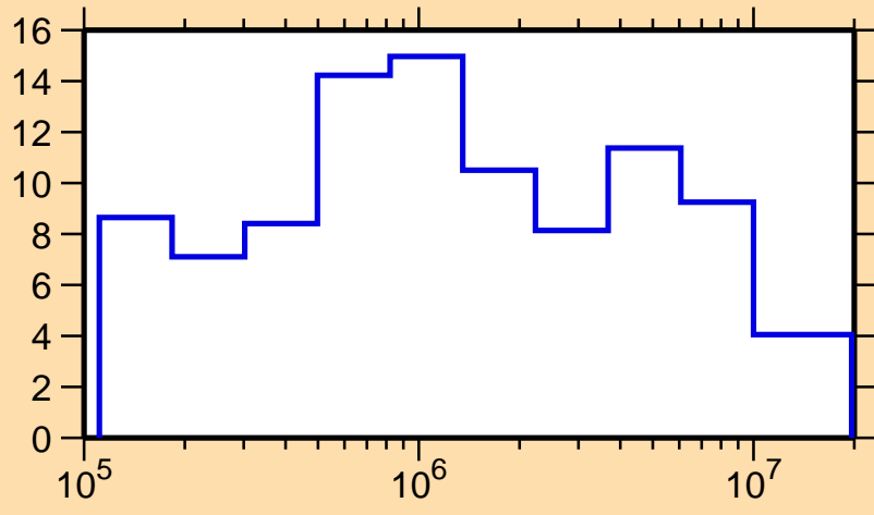
\Delta\sigma/\sigma vs. E for ^{188}\text{Hf}(n,\text{tot.})
