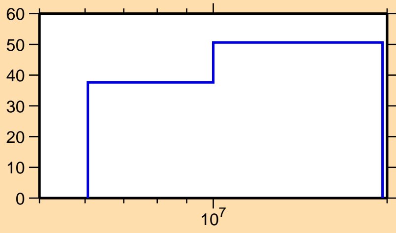
\Delta\sigma/\sigma vs. E for ^{188}\text{Hf}(n,n\text{cont.})
