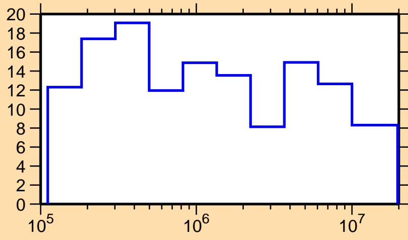
\Delta\sigma/\sigma vs. E for ^{188}\text{Hf}(n,\text{el.})
