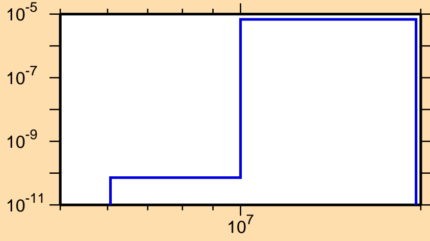
\sigma vs. E for ^{188}\text{Hf}(n,\alpha)
