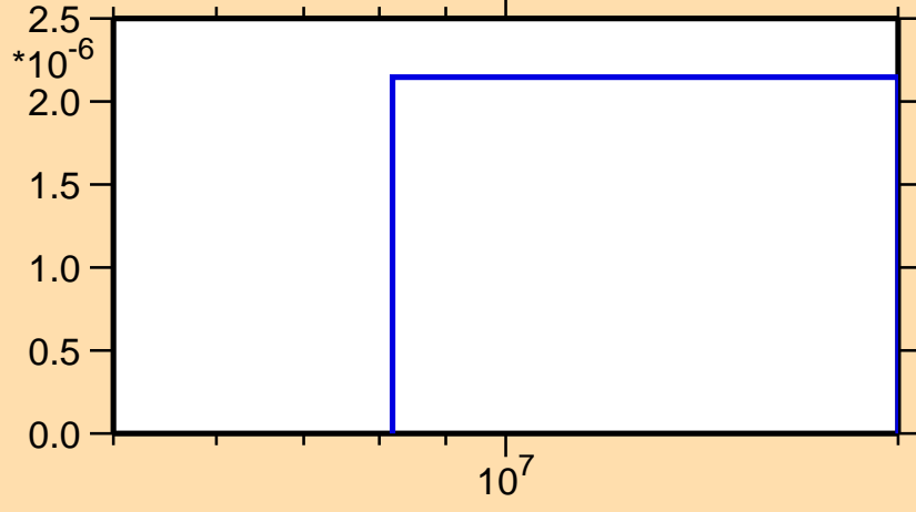
\sigma vs. E for ^{188}\text{Hf}(n,t)
