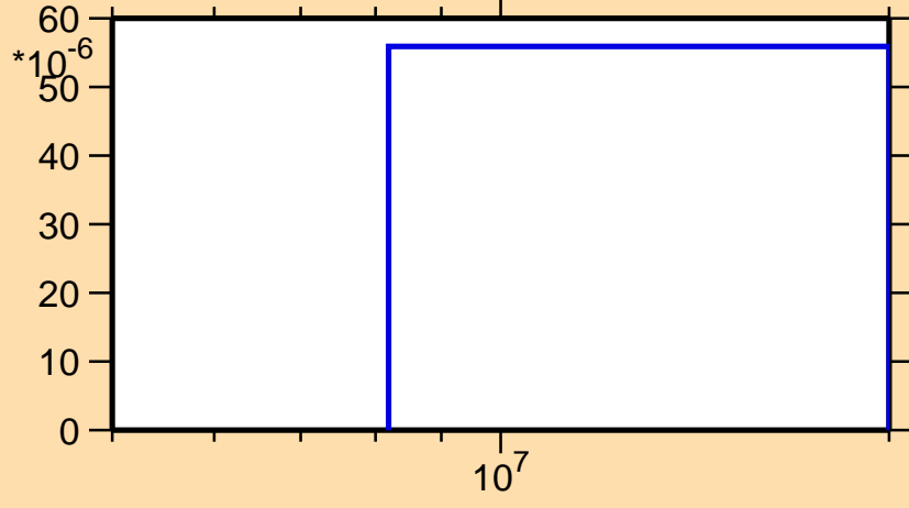
\sigma vs. E for ^{188}\text{Hf}(n,p)
