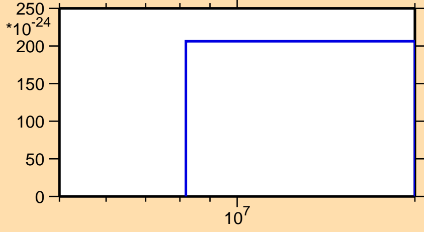
\sigma vs. E for ^{188}\text{Hf}(\text{mt } 11)
