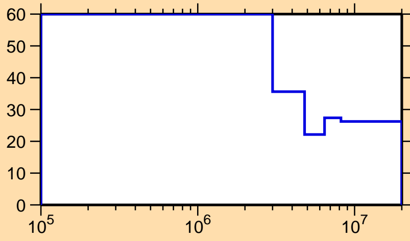
\Delta\sigma/\sigma vs. E for ^{188}\text{Hf}(n,n_1)
