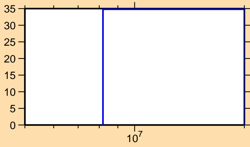
\Delta\sigma/\sigma vs. E for ^{188}\text{Hf}(n,2n)
