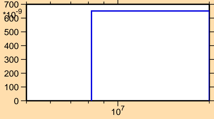
\sigma vs. E for ^{188}\text{Hf}(n,n\alpha)
