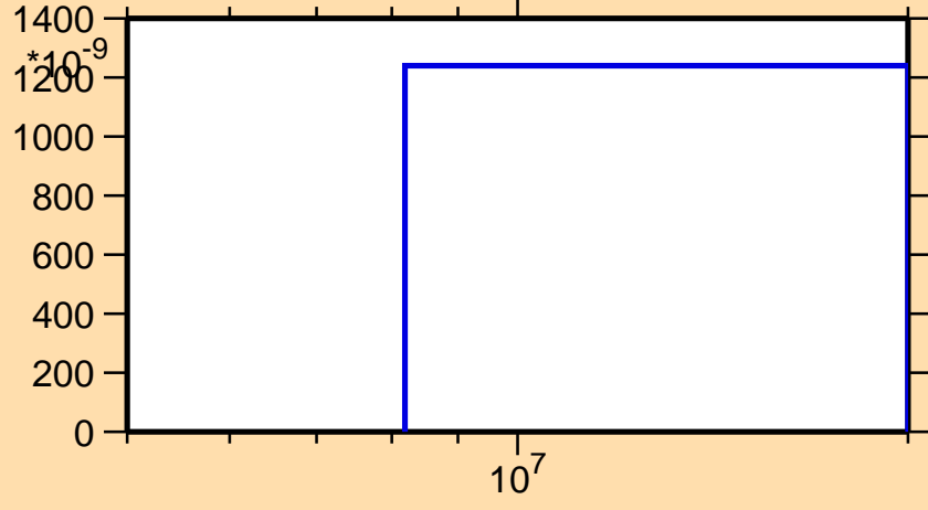
\sigma vs. E for ^{188}\text{Hf}(n,d)
