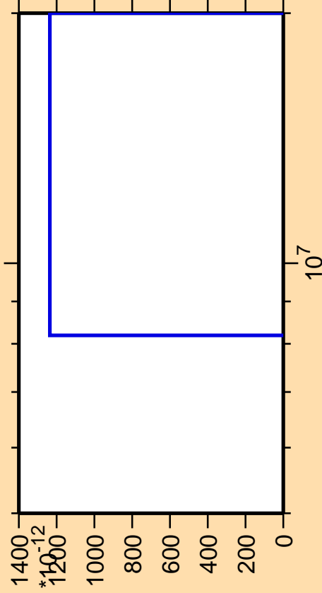
\Delta\sigma/\sigma vs. E for ^{188}\text{Hf}(\text{mt } 11)
