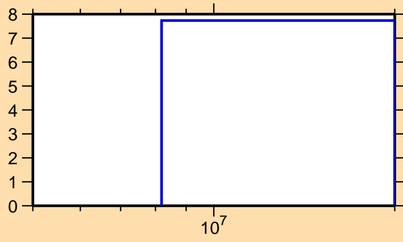
\Delta\sigma/\sigma vs. E for ^{188}\text{Hf}(n,el.)
