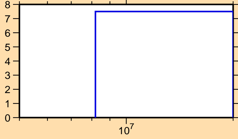
\Delta\sigma/\sigma vs. E for ^{188}\text{Hf}(n,\text{nonel.})
