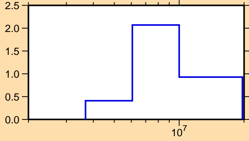
\sigma vs. E for ^{189}\text{Hf}(n,2n)
