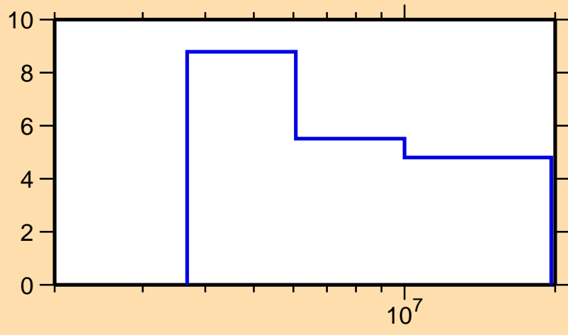
\Delta\sigma/\sigma vs. E for ^{189}\text{Hf}(n,\text{nonel.})
