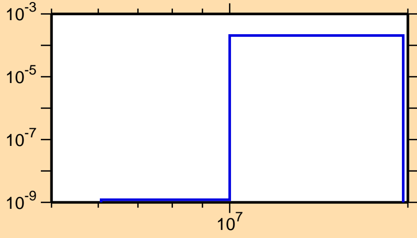
\sigma vs. E for ^{189}\text{Hf}(n,p)
