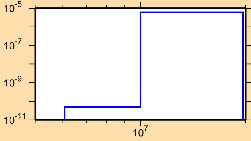
\sigma vs. E for ^{189}\text{Hf}(n,\alpha)
