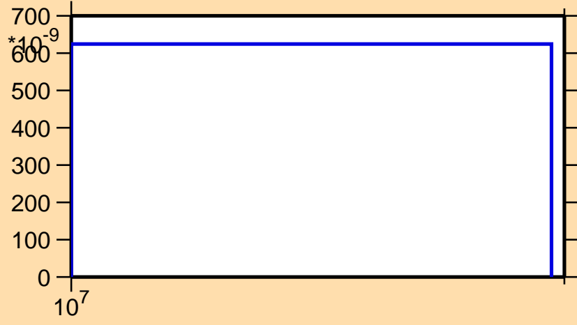
\sigma vs. E for ^{189}\text{Hf}(n,np)
