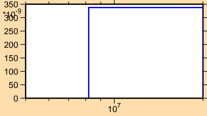
\sigma vs. E for ^{189}\text{Hf}(n,n\alpha)
