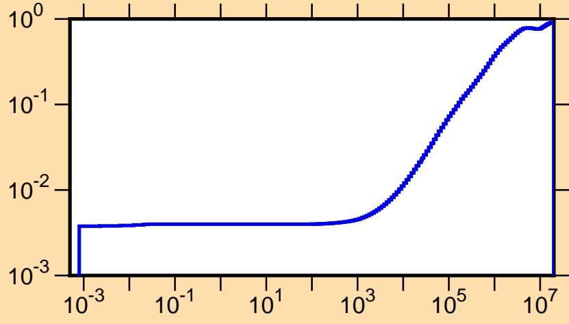
\mu vs. E for ^{179}\text{Hg}(\text{mt251})
