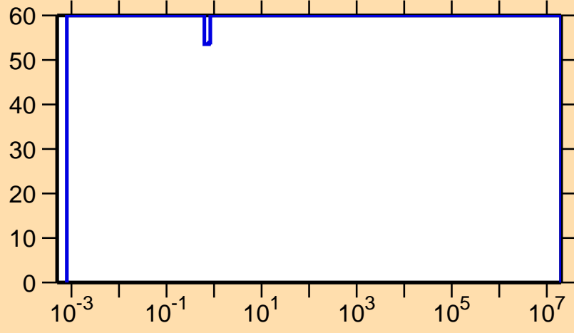
\Delta\sigma/\sigma vs. E for ^{179}\text{Hg}(n,\gamma)
