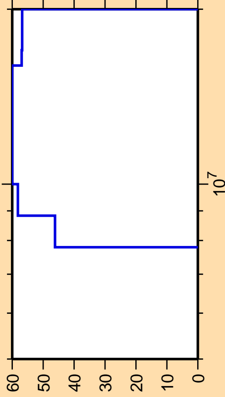
\Delta\sigma/\sigma vs. E for ^{179}\text{Hg}(n,n\text{cont.})
