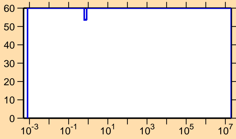
\Delta\sigma/\sigma vs. E for ^{179}\text{Hg}(n,\gamma)
