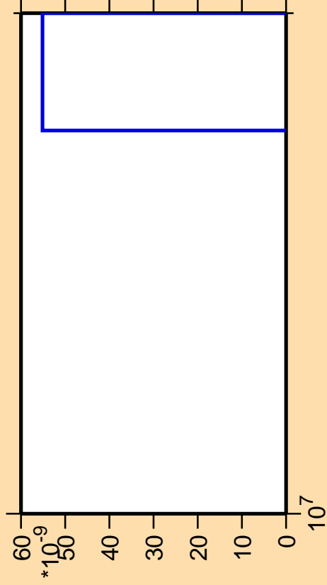
\Delta\sigma/\sigma vs. E for ^{179}\text{Hg} (mt 11)
