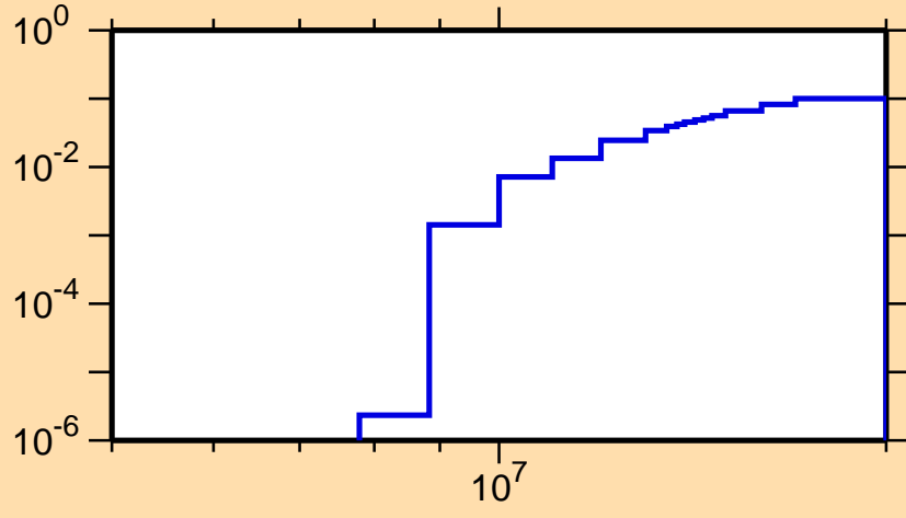
\sigma vs. E for ^{179}\text{Hg}(n,2n)
