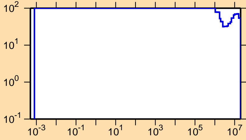
\Delta\sigma/\sigma vs. E for ^{179}\text{Hg}(n,p)
