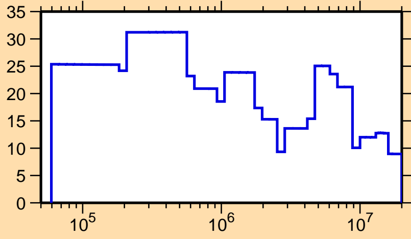
\Delta\sigma/\sigma vs. E for ^{179}\text{Hg}(n,\text{el.})
