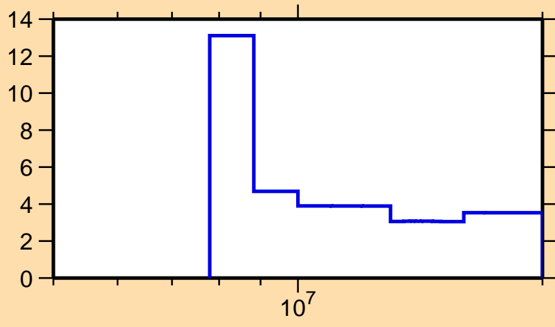
\Delta\sigma/\sigma vs. E for ^{179}\text{Hg}(n,\text{tot.})
