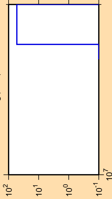
\Delta\sigma/\sigma vs. E for ^{179}\text{Hg}(n,nt)
