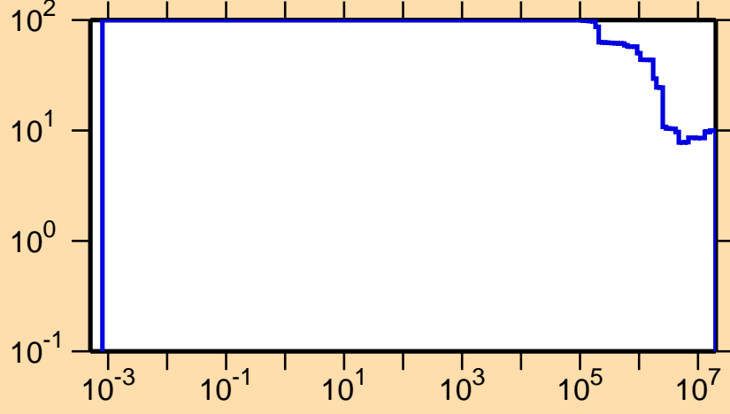
\Delta\sigma/\sigma vs. E for ^{179}\text{Hg}(n,\text{nonel.})
