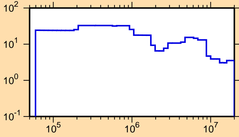
\Delta\sigma/\sigma vs. E for ^{179}\text{Hg}(n,\text{tot.})
