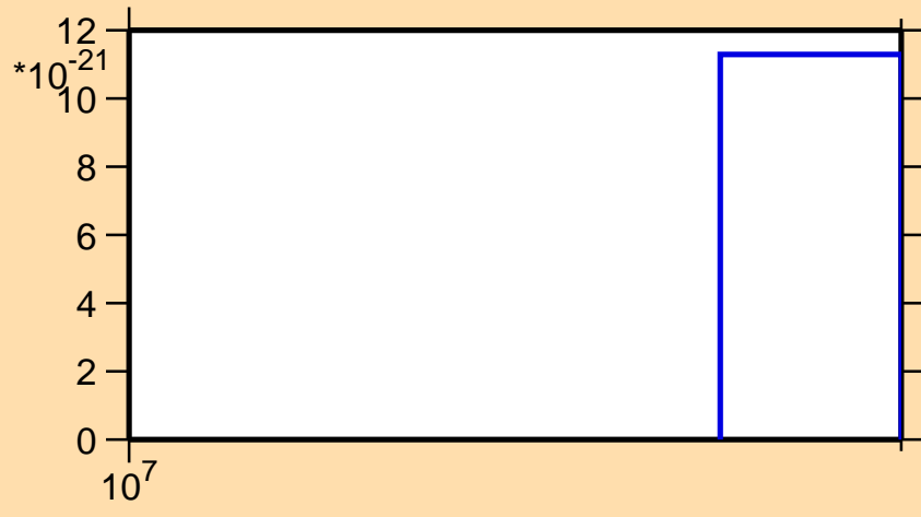
\sigma vs. E for ^{179}\text{Hg} (mt 11)
