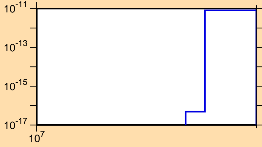
\sigma vs. E for ^{179}\text{Hg}(n,nt)
