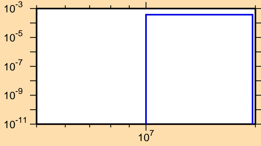
\sigma vs. E for ^{179}\text{Hg}(n,2n\alpha)
