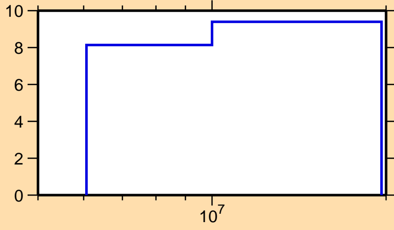
\Delta\sigma/\sigma vs. E for ^{179}\text{Hg}(n,\text{nonel.})
