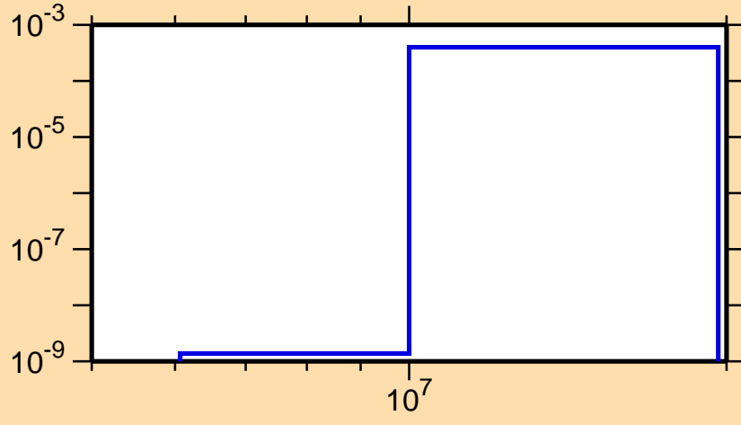
\sigma vs. E for ^{179}\text{Hg}(n,t)
