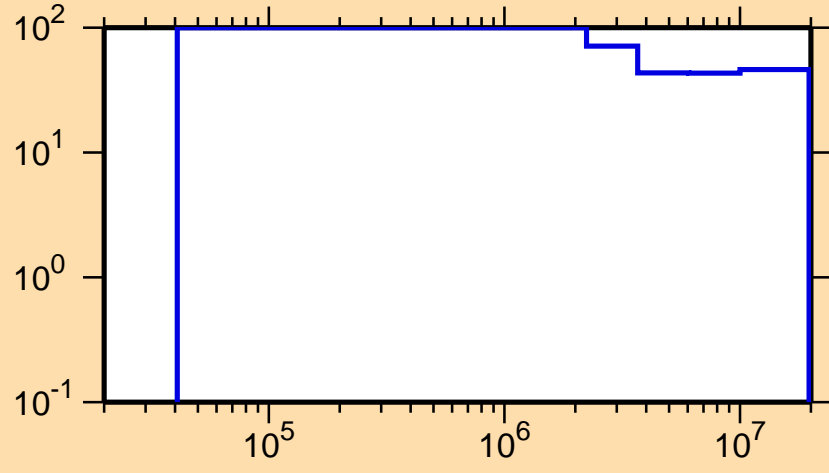
\Delta\sigma/\sigma vs. E for ^{179}\text{Hg}(n,n_1)
