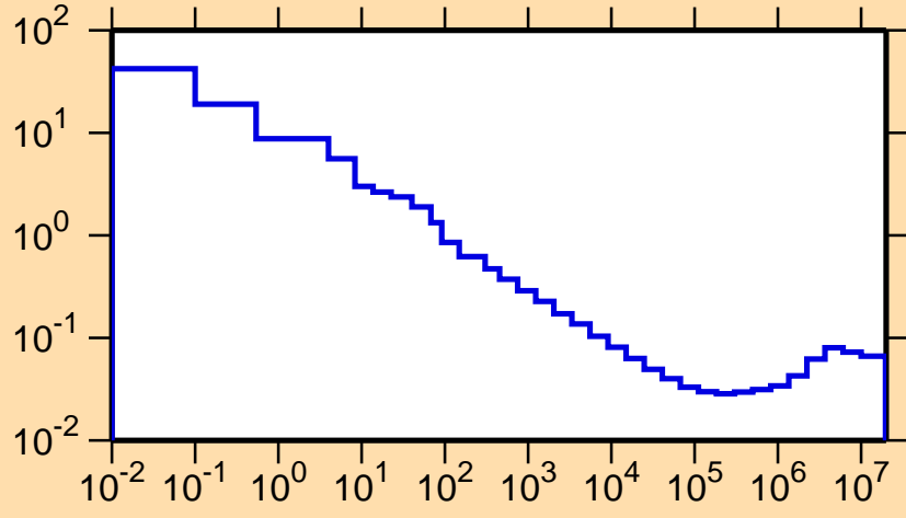
\sigma vs. E for ^{179}\text{Hg}(n,p\alpha)
