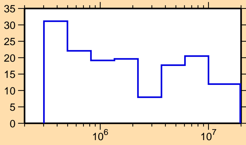
\Delta\sigma/\sigma vs. E for ^{179}\text{Hg}(n,\text{el.})
