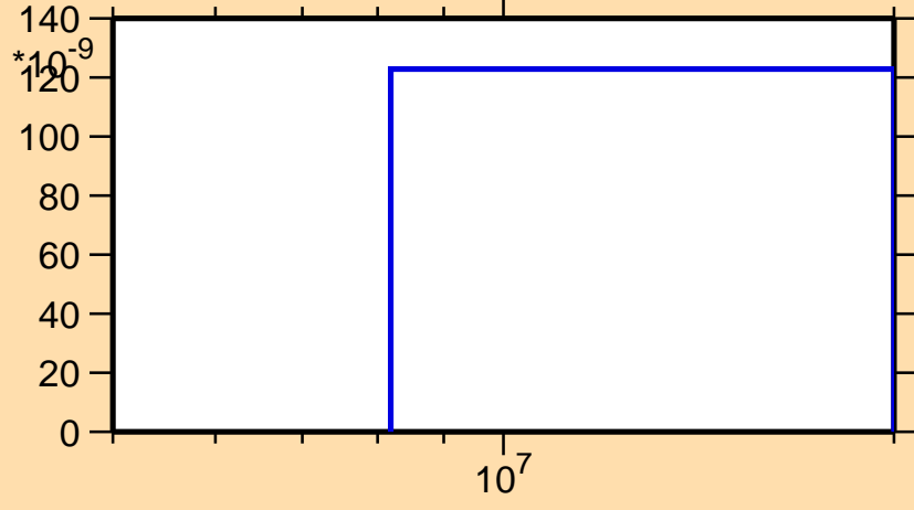
\sigma vs. E for ^{179}\text{Hg}(n,\text{nd})
