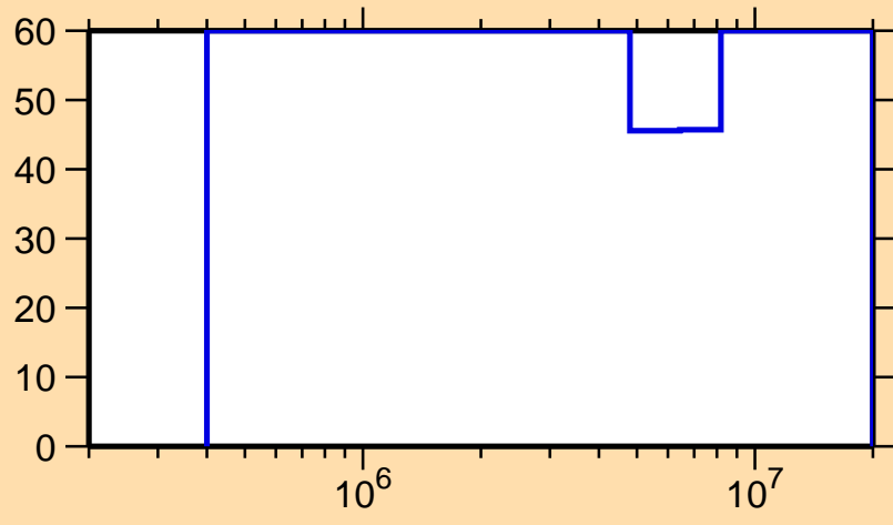
\Delta\sigma/\sigma vs. E for ^{179}\text{Hg}(n,n\text{cont.})
