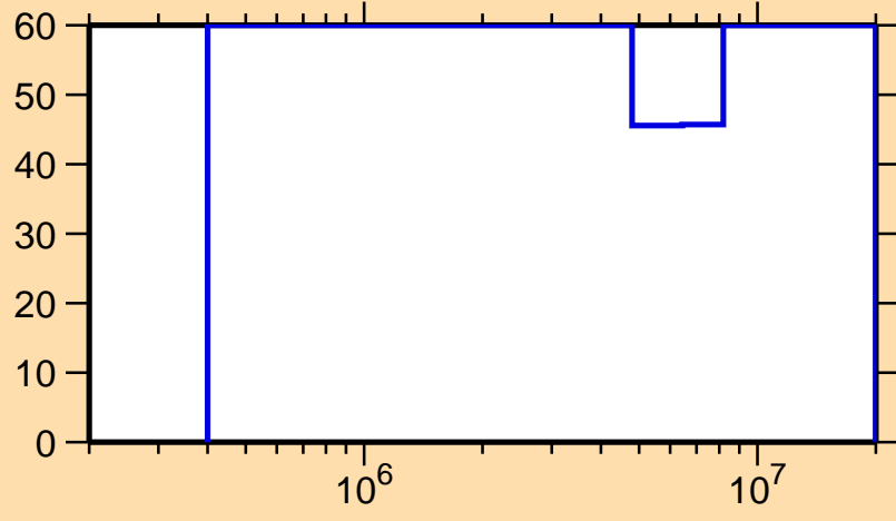
\Delta\sigma/\sigma vs. E for ^{179}\text{Hg}(n,n\text{cont.})
