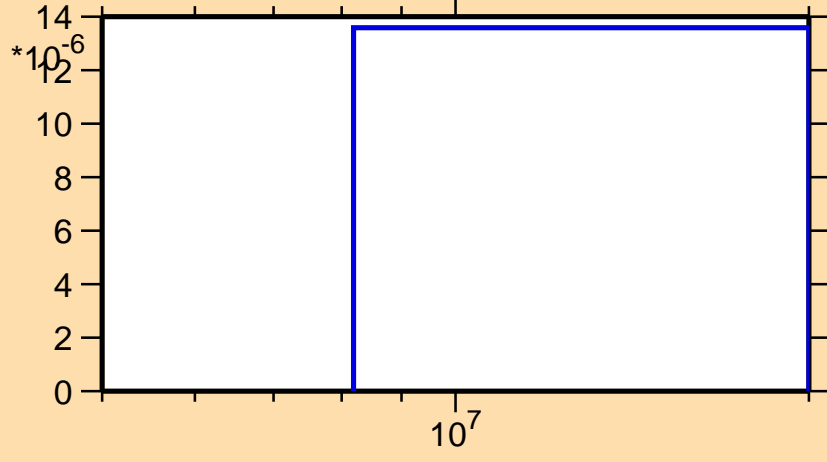
\sigma vs. E for ^{180}\text{Hg}(n,2n\alpha)
