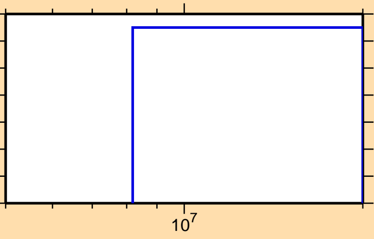
\sigma vs. E for ^{180}\text{Hg}(n,2n)
