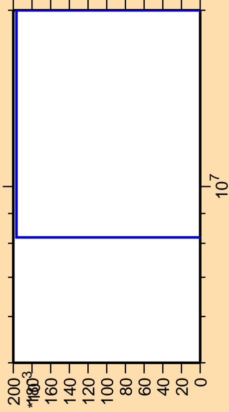
\Delta\sigma/\sigma vs. E for ^{180}\text{Hg}(n,nt)
