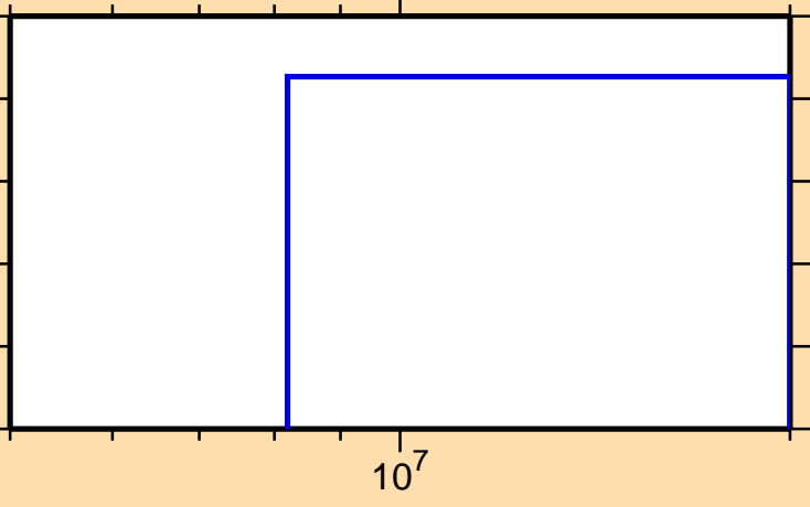
\sigma vs. E for ^{180}\text{Hg}(n,\text{nd})
