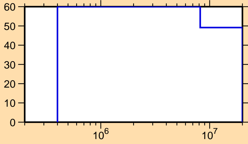
\Delta\sigma/\sigma vs. E for ^{180}\text{Hg}(n,n_1)
