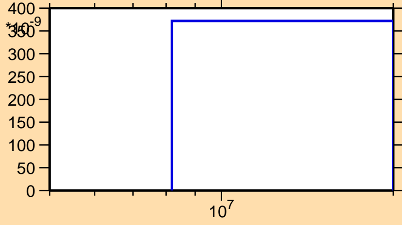
\sigma vs. E for ^{180}\text{Hg}(n,2np)
