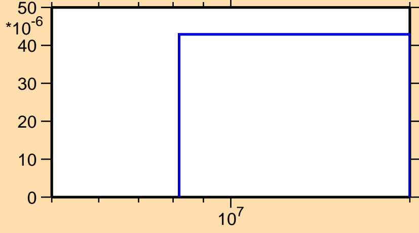
\sigma vs. E for ^{180}\text{Hg}(n,t)
