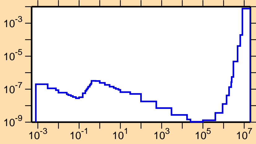
\sigma vs. E for ^{180}\text{Hg}(n,p\alpha)
