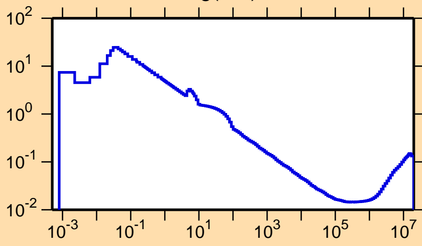
\sigma vs. E for ^{181}\text{Hg}(n,\alpha)
