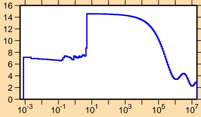
\sigma vs. E for ^{181}\text{Hg}(n,\text{el.})
