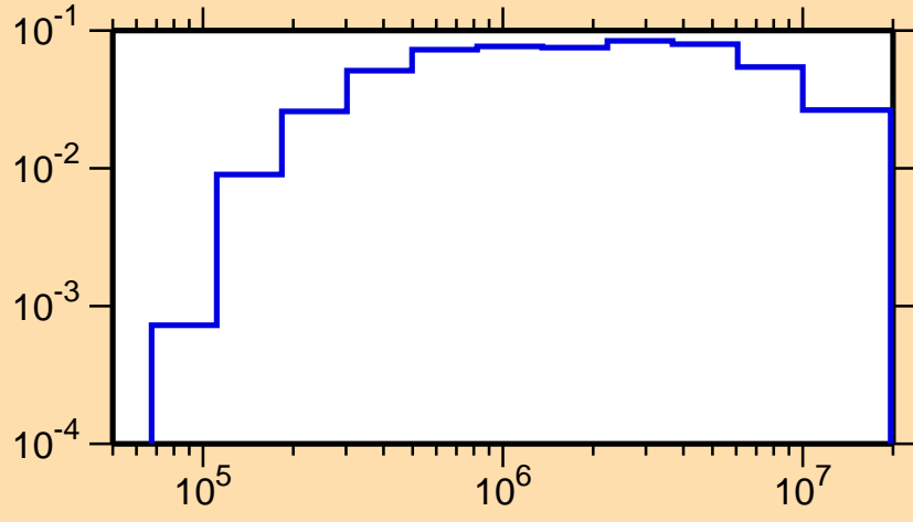
\sigma vs. E for ^{181}\text{Hg}(n,n_2)
