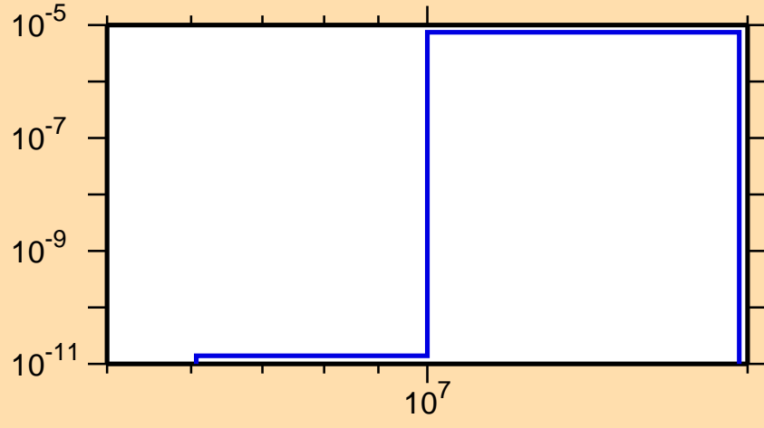
\sigma vs. E for ^{181}\text{Hg}(n,\text{pd})
