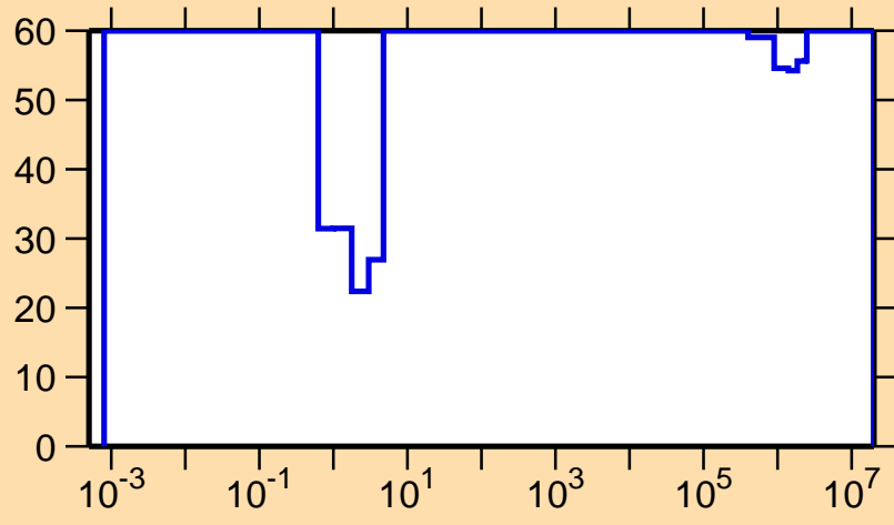
\Delta\sigma/\sigma vs. E for ^{181}\text{Hg}(n,\gamma)
