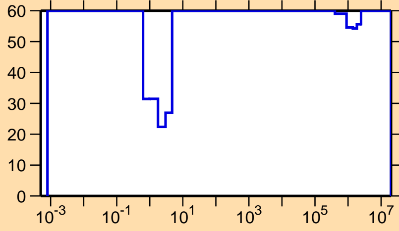
\Delta\sigma/\sigma vs. E for ^{181}\text{Hg}(n,\gamma)
