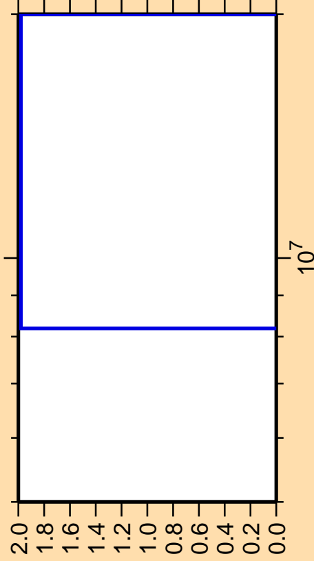
\Delta\sigma/\sigma vs. E for ^{181}\text{Hg}(n,nt)
