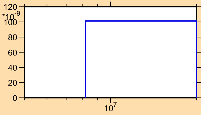
\sigma vs. E for ^{181}\text{Hg}(n,\text{nd})
