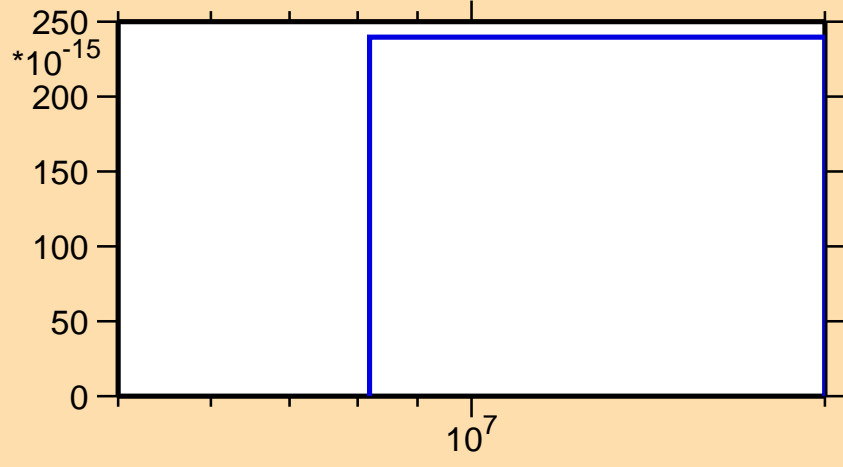
\sigma vs. E for ^{181}\text{Hg}(n,nt)
