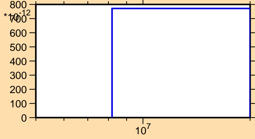
\sigma vs. E for ^{181}\text{Hg} (mt 34)
