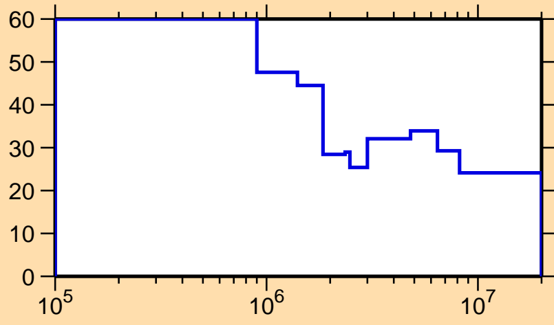
\Delta\sigma/\sigma vs. E for ^{181}\text{Hg}(n,n_1)
