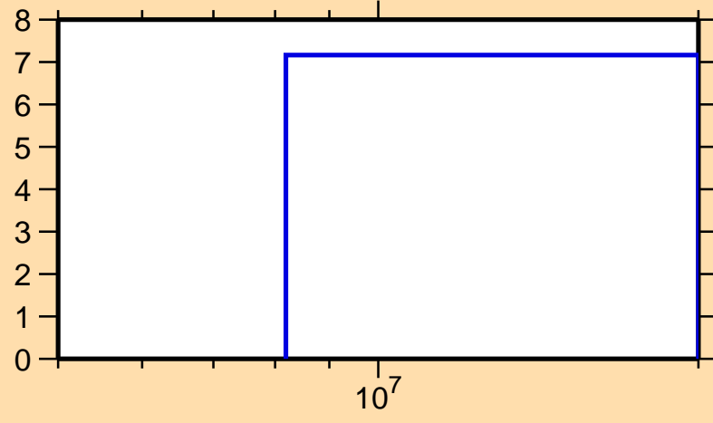
\Delta\sigma/\sigma vs. E for ^{181}\text{Hg}(n,\text{nonel.})
