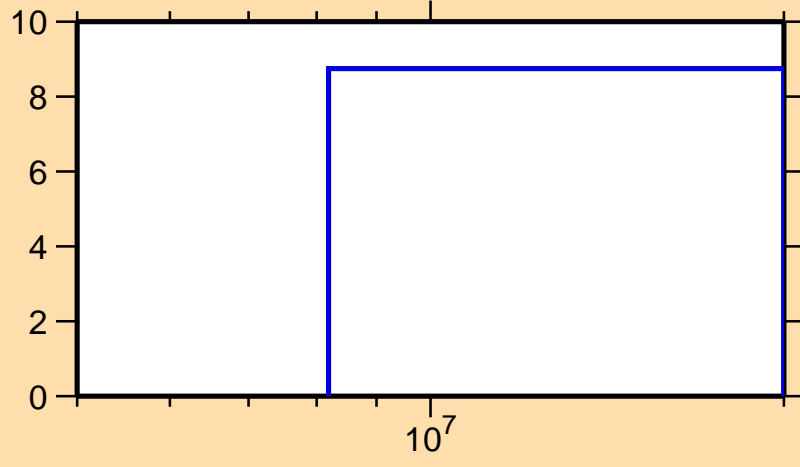
\Delta\sigma/\sigma vs. E for ^{181}\text{Hg}(n,\text{el.})
