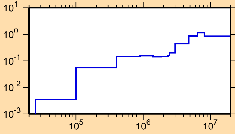
\sigma vs. E for ^{181}\text{Hg}(n,\text{inel.})
