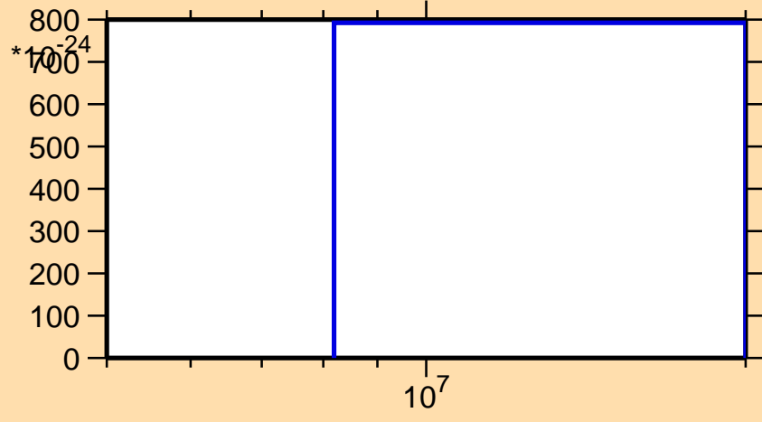
\sigma vs. E for ^{181}\text{Hg} (mt 11)
