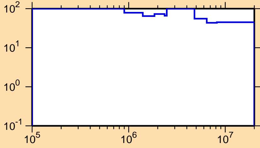
\Delta\sigma/\sigma vs. E for ^{181}\text{Hg}(n,n\text{cont.})
