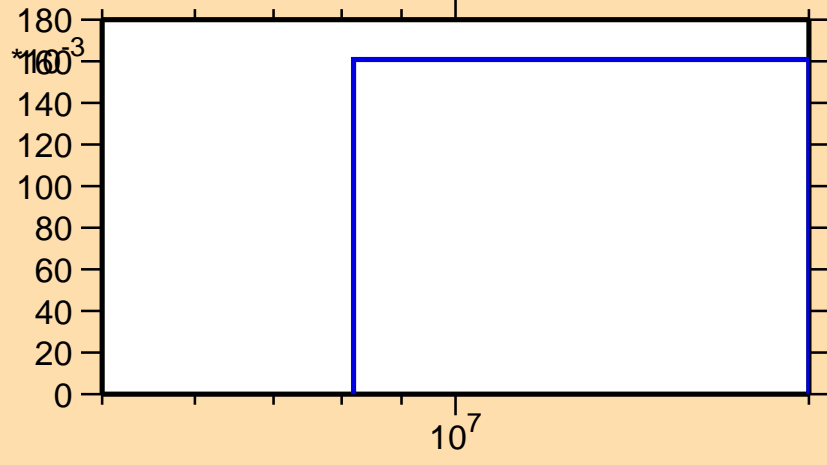
\sigma vs. E for ^{181}\text{Hg}(n,2n)
