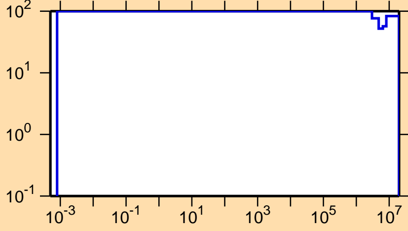
\Delta\sigma/\sigma vs. E for ^{181}\text{Hg}(n,p)
