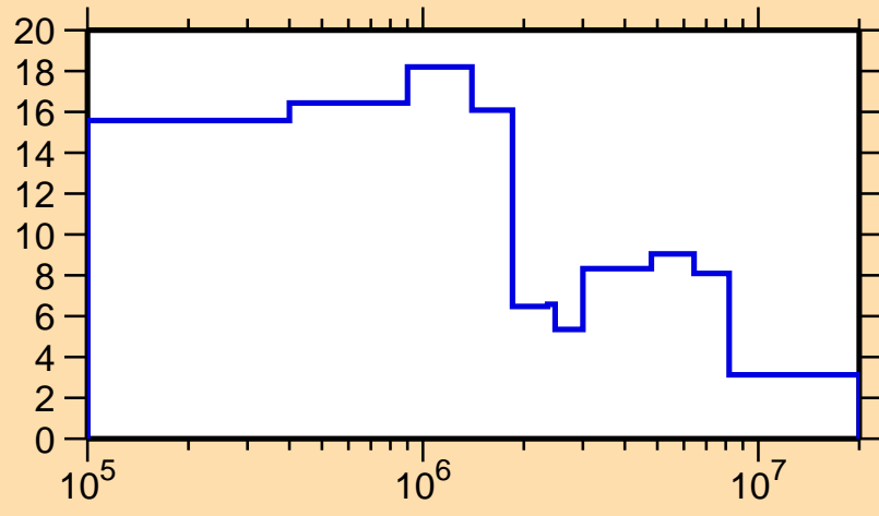
\Delta\sigma/\sigma vs. E for ^{181}\text{Hg}(n,\text{tot.})
