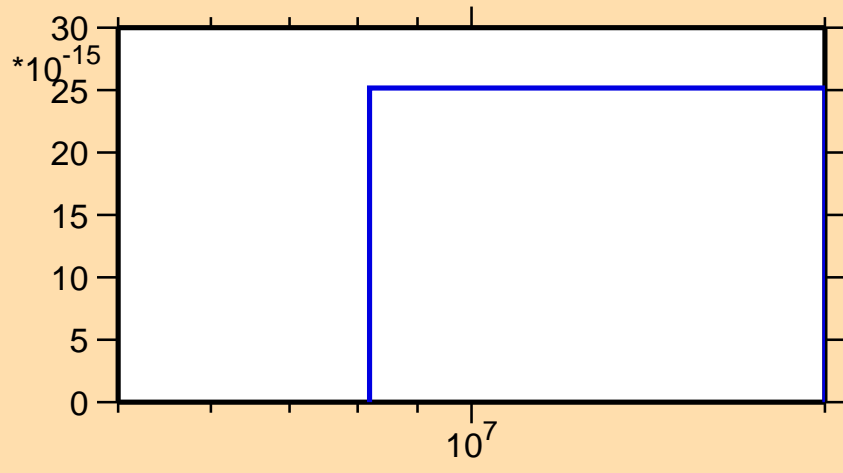
\sigma vs. E for ^{181}\text{Hg}(n,3n)
