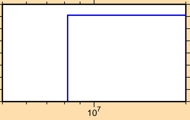
\sigma vs. E for ^{181}\text{Hg}(n,\text{pt})
