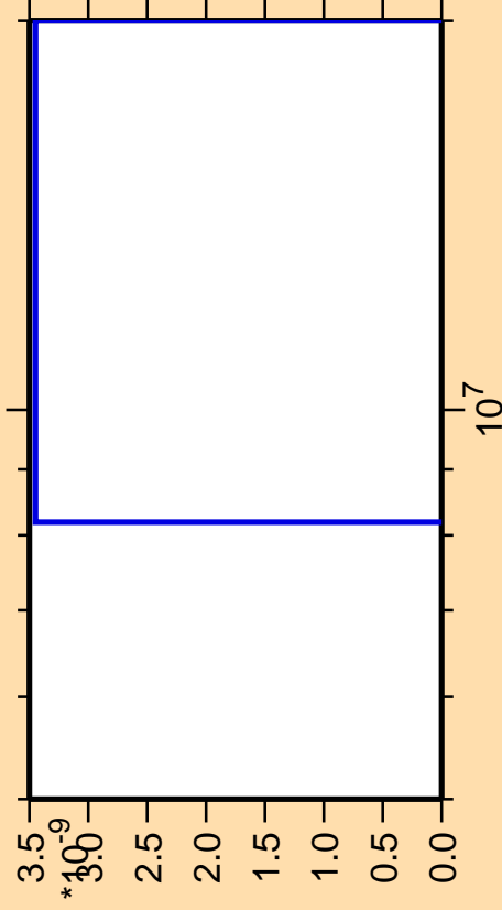
\Delta\sigma/\sigma vs. E for ^{181}\text{Hg} (mt 11)
