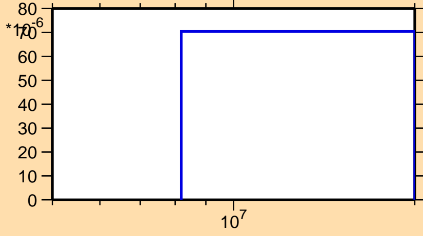
\sigma vs. E for ^{181}\text{Hg}(n,2n\alpha)
