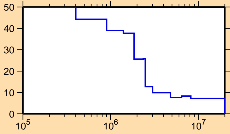
\Delta\sigma/\sigma vs. E for ^{181}\text{Hg}(n,\text{nonel.})
