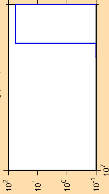
\Delta\sigma/\sigma vs. E for ^{182}\text{Hg}(n,nt)
