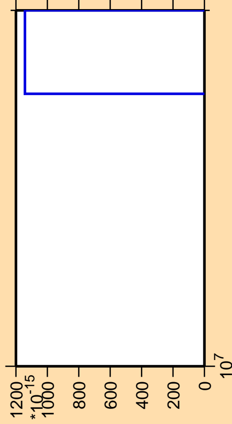
\Delta\sigma/\sigma vs. E for ^{182}\text{Hg} (mt 11)
