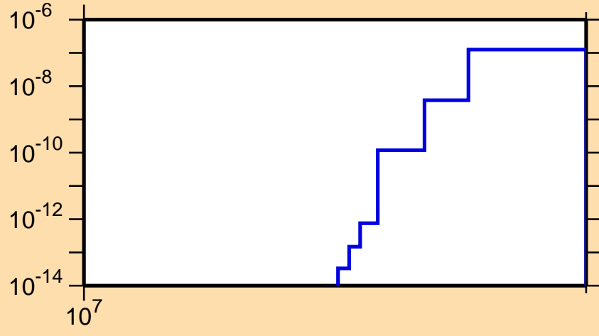
\sigma vs. E for ^{182}\text{Hg}(n,\text{nd})
