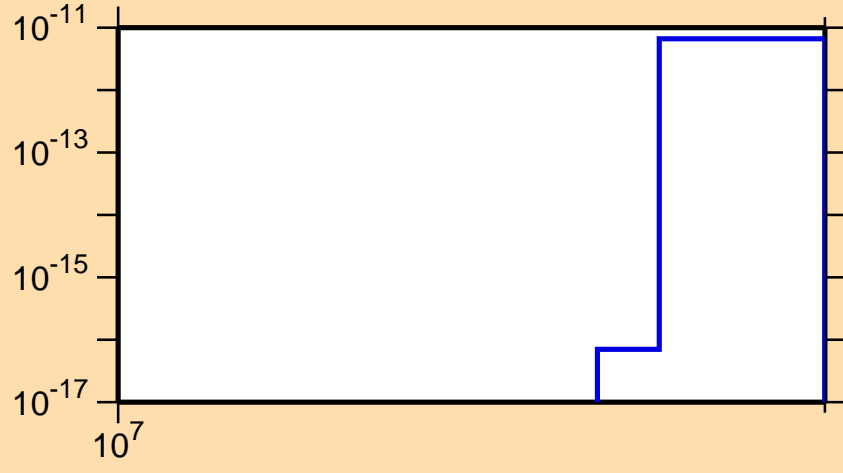
\sigma vs. E for ^{182}\text{Hg}(n,nt)
