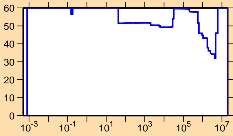
\Delta\sigma/\sigma vs. E for ^{182}\text{Hg}(n,\gamma)
