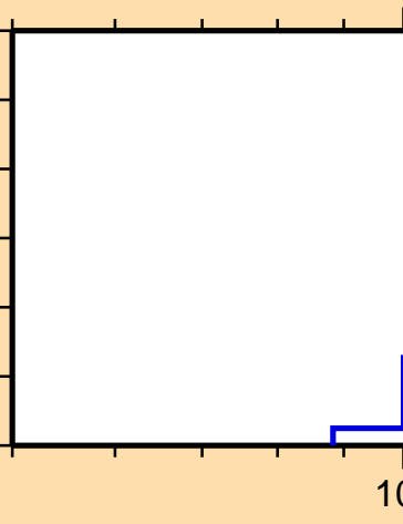
\sigma vs. E for ^{182}\text{Hg}(\text{mt117})
