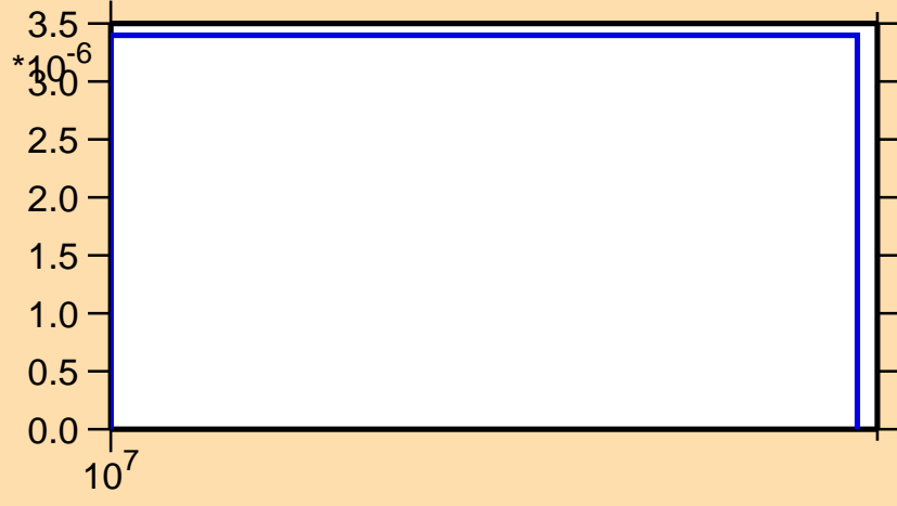
\sigma vs. E for ^{182}\text{Hg}(n,2n\alpha)
