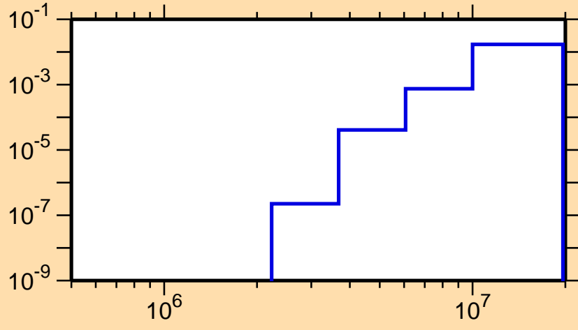
\sigma vs. E for ^{182}\text{Hg}(n,n\alpha)
