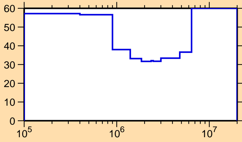
\Delta\sigma/\sigma vs. E for ^{182}\text{Hg}(n,n_1)
