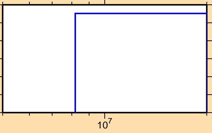
\sigma vs. E for ^{182}\text{Hg} (mt 11)
