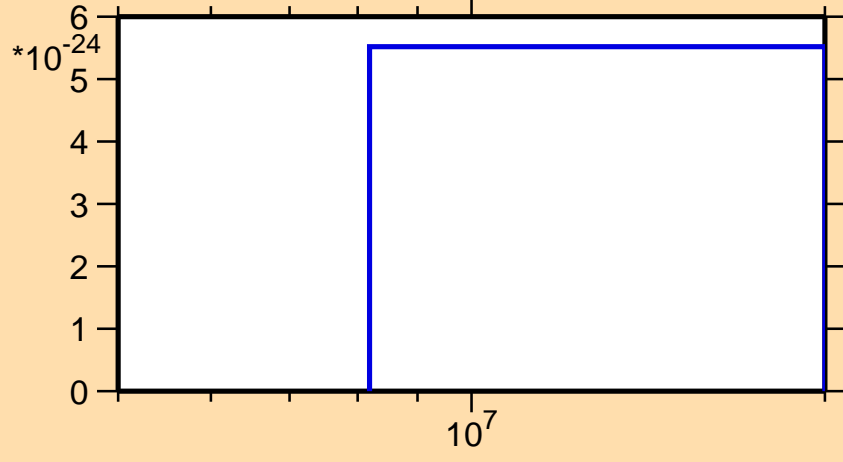
\sigma vs. E for ^{182}\text{Hg} (mt 11)
