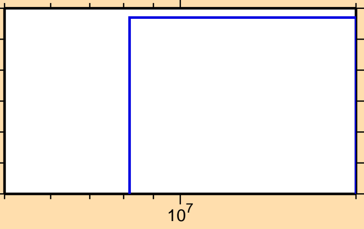
\sigma vs. E for ^{182}\text{Hg}(\text{mt117})
