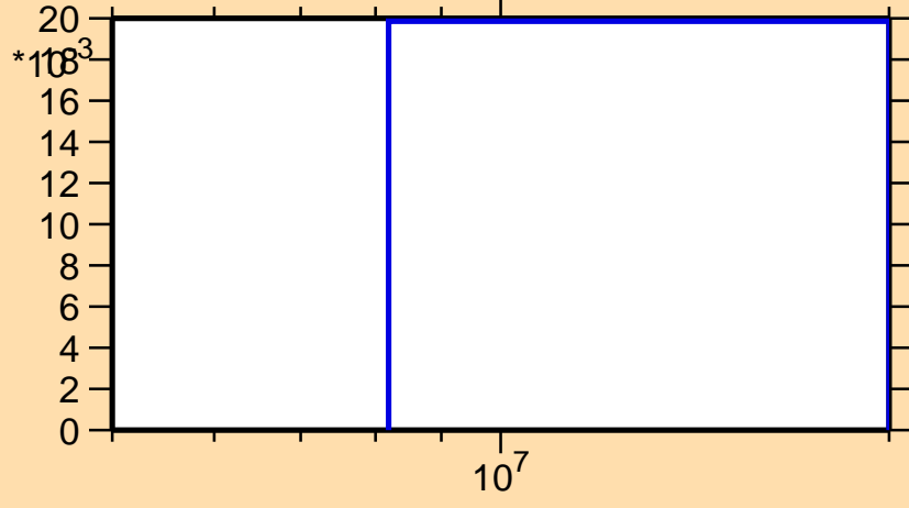
\sigma vs. E for ^{182}\text{Hg}(n,2n)
