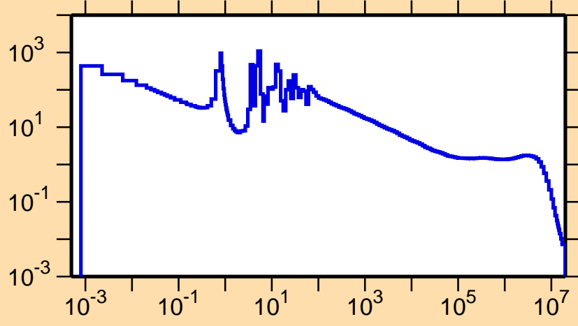
\sigma vs. E for ^{184}\text{Hg}(n,\gamma)
