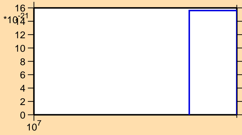
\sigma vs. E for ^{184}\text{Hg} (mt 11)
