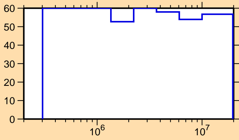
\Delta\sigma/\sigma vs. E for ^{184}\text{Hg}(n,\text{inel.})
