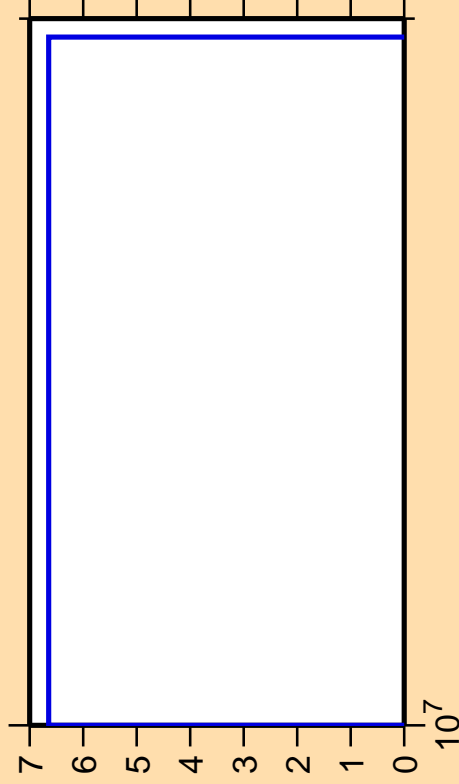
\Delta\sigma/\sigma vs. E for ^{184}\text{Hg} (mt 34)
