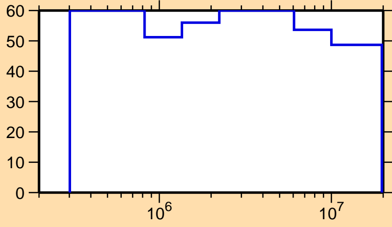
\Delta\sigma/\sigma vs. E for ^{184}\text{Hg}(n,n_1)
