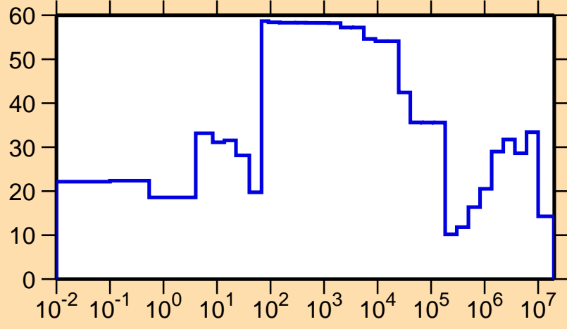
\Delta\sigma/\sigma vs. E for ^{184}\text{Hg}(n,\text{el.})
