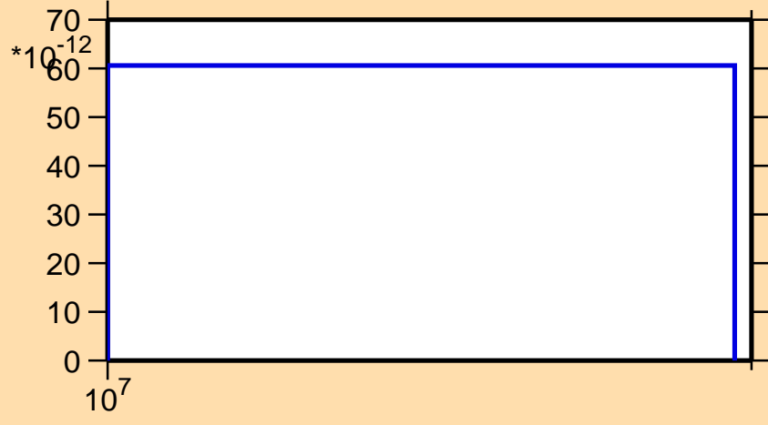
\sigma vs. E for ^{184}\text{Hg}(n,\text{pt})
