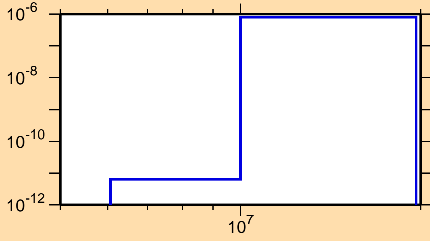
\sigma vs. E for ^{184}\text{Hg}(n,\text{He}3)
