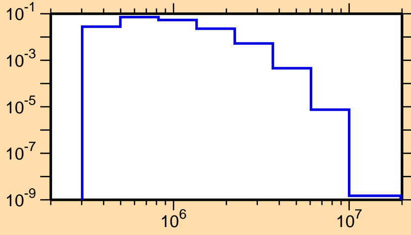
\sigma vs. E for ^{184}\text{Hg}(n,n_2)
