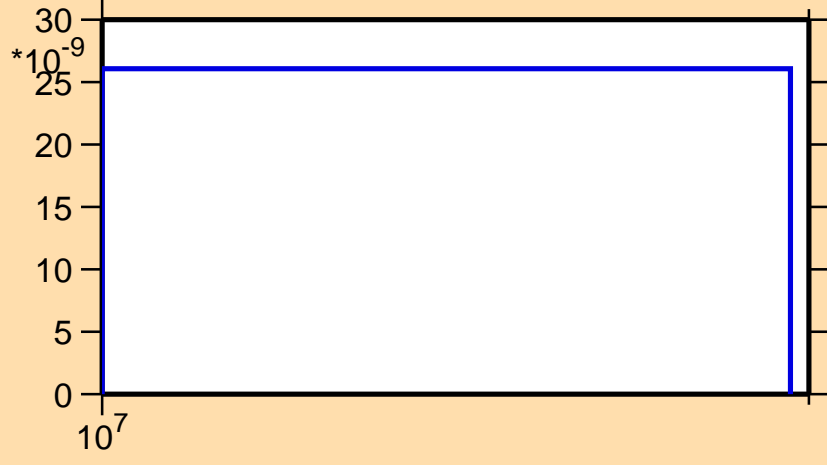
\sigma vs. E for ^{184}\text{Hg}(n,3n)
