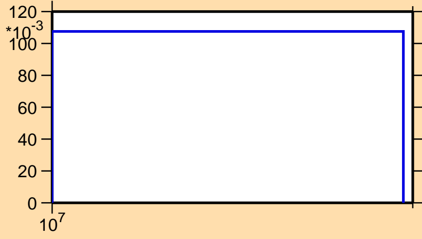
\sigma vs. E for ^{184}\text{Hg}(n,2n)
