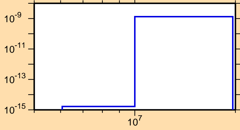
\sigma vs. E for ^{184}\text{Hg}(\text{mt117})
