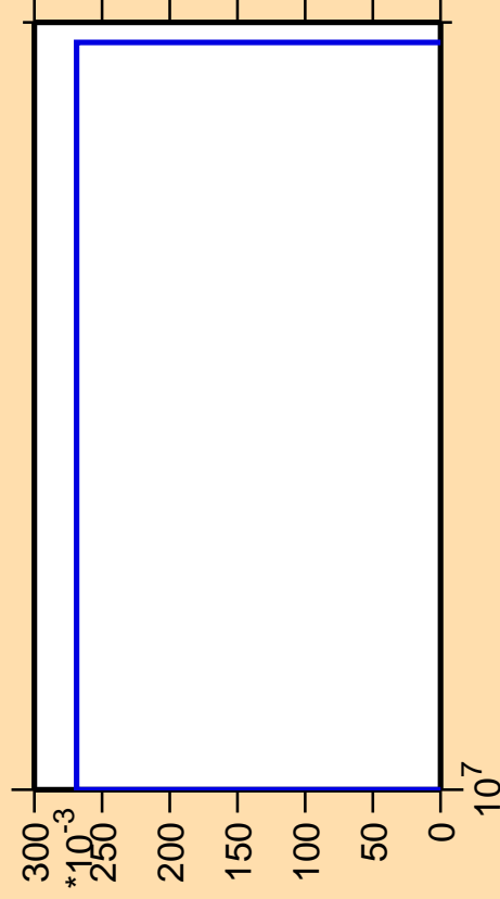
\Delta\sigma/\sigma vs. E for ^{184}\text{Hg}(n,nt)
