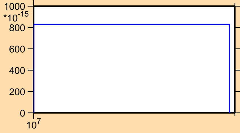
\sigma vs. E for ^{184}\text{Hg} (mt 34)
