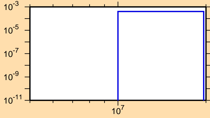
\sigma vs. E for ^{184}\text{Hg}(n,2n\alpha)
