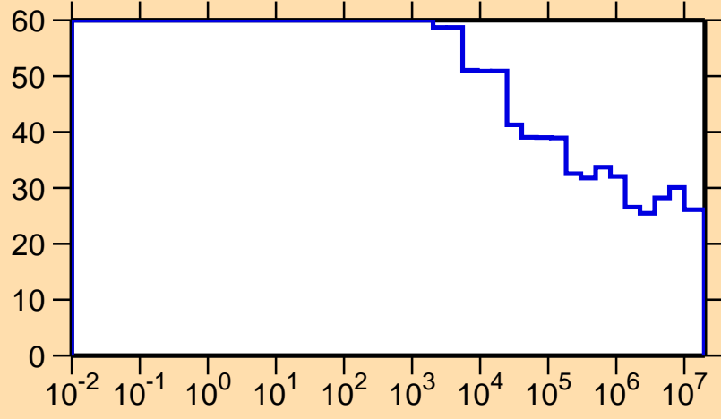
\Delta\sigma/\sigma vs. E for ^{184}\text{Hg}(n,\text{nonel.})
