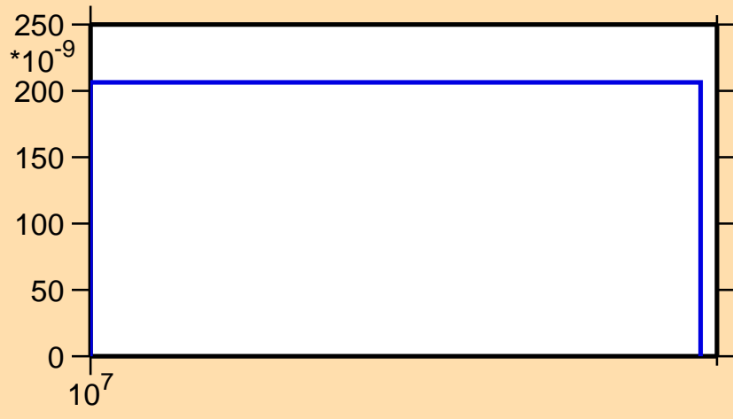
\sigma vs. E for ^{184}\text{Hg}(n,2np)
