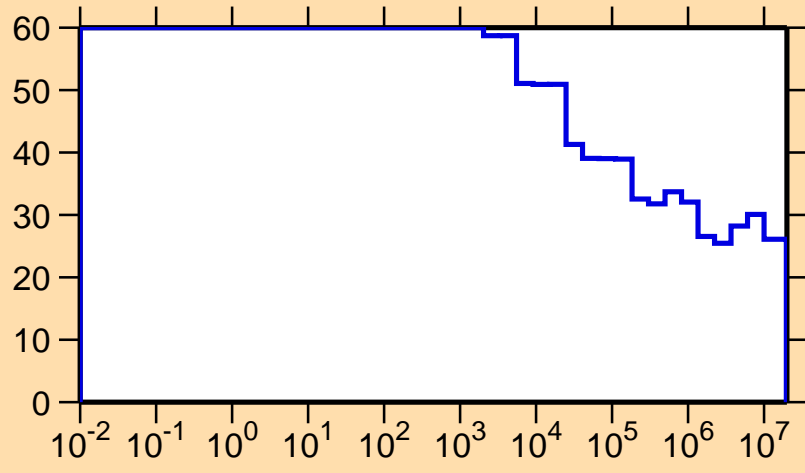
\Delta\sigma/\sigma vs. E for ^{184}\text{Hg}(n,\text{nonel.})
