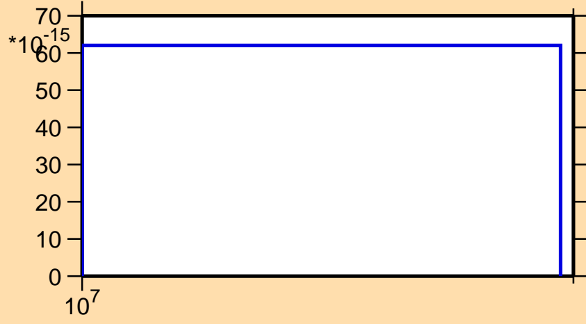
\sigma vs. E for ^{184}\text{Hg}(n,nt)
