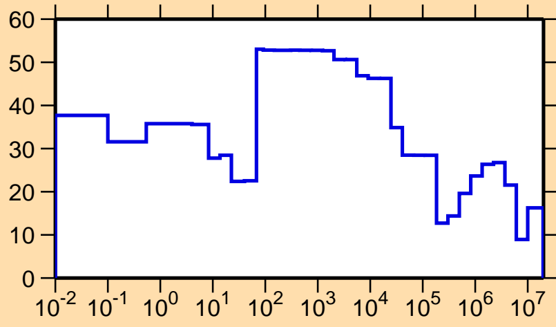
\Delta\sigma/\sigma vs. E for ^{184}\text{Hg}(n,\text{tot.})
