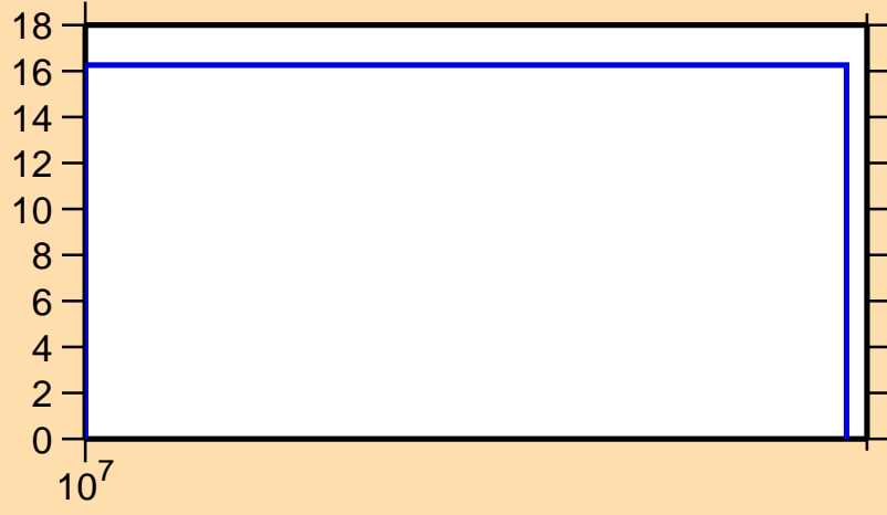
\Delta\sigma/\sigma vs. E for ^{184}\text{Hg}(n,\text{tot.})
