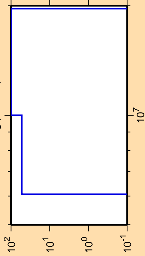
\Delta\sigma/\sigma vs. E for ^{184}\text{Hg}(n,\text{He}3)
