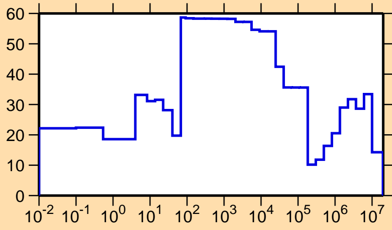
\Delta\sigma/\sigma vs. E for ^{184}\text{Hg}(n,\text{el.})
