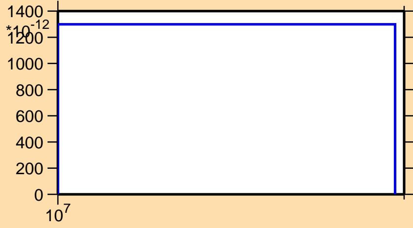
\sigma vs. E for ^{184}\text{Hg}(n,\text{nd})
