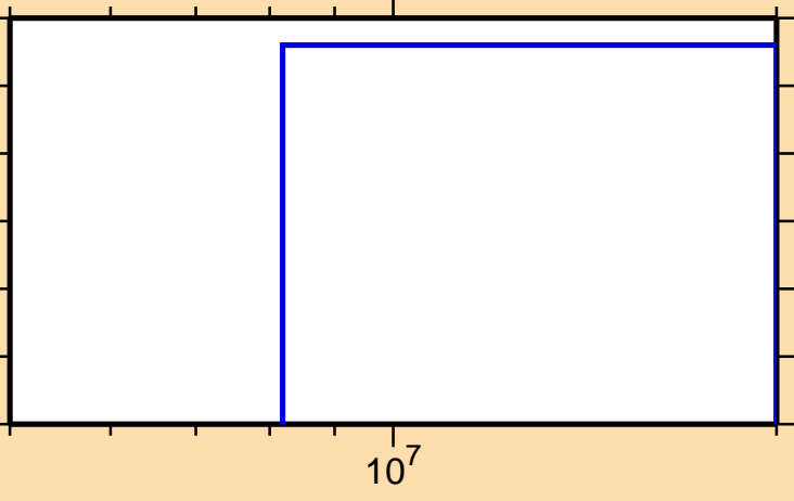
\sigma vs. E for ^{184}\text{Hg}(n,\text{pt})
