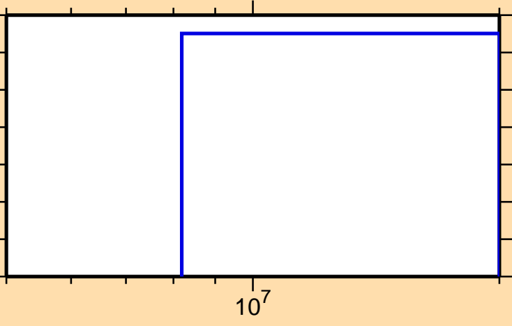
\sigma vs. E for ^{184}\text{Hg}(n,\text{pd})
