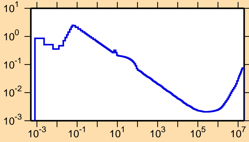
\sigma vs. E for ^{185}\text{Hg}(n,\alpha)
