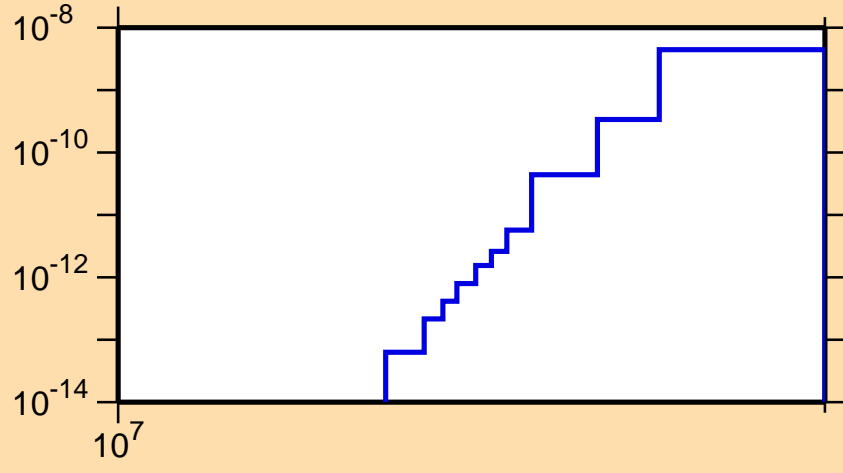
\sigma vs. E for ^{185}\text{Hg} (mt 34)
