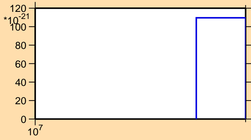
\sigma vs. E for ^{185}\text{Hg} (mt 11)
