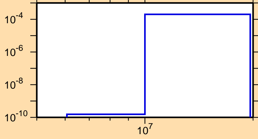
\sigma vs. E for ^{185}\text{Hg}(n,t)
