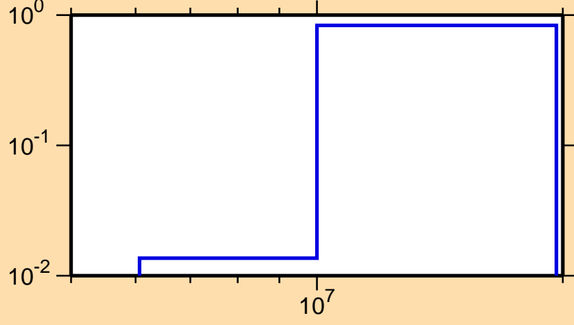
\sigma vs. E for ^{185}\text{Hg}(n,2n)
