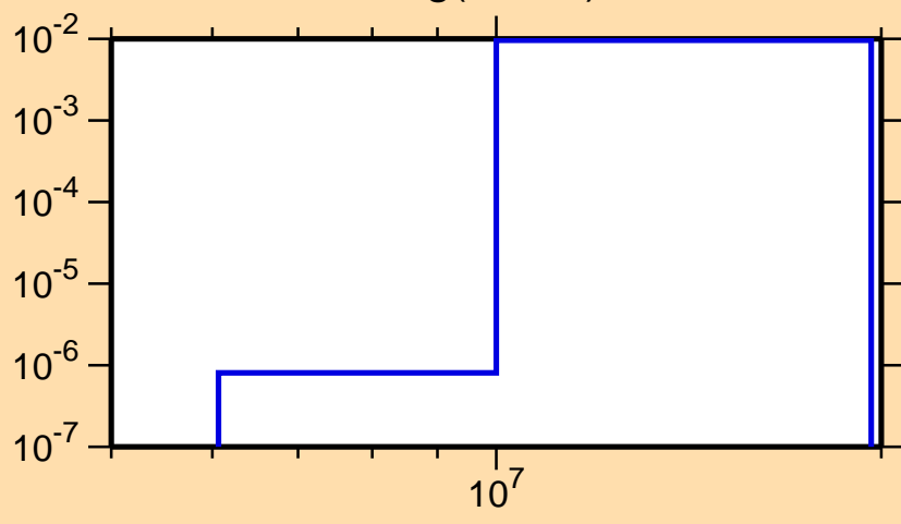
\sigma vs. E for ^{185}\text{Hg}(n,2n\alpha)
