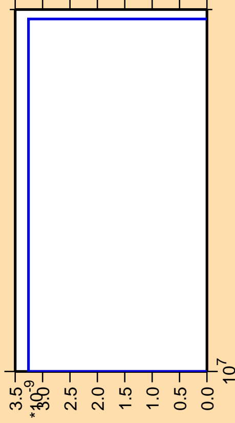
\Delta\sigma/\sigma vs. E for ^{185}\text{Hg} (mt 11)
