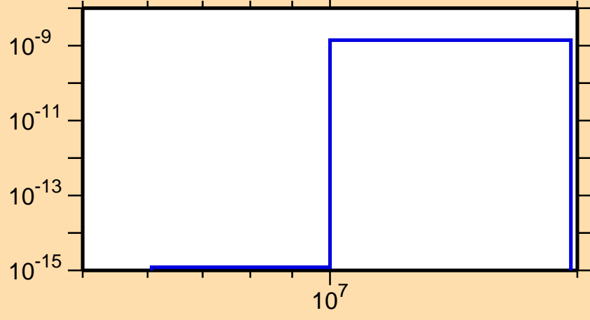
\sigma vs. E for ^{185}\text{Hg}(\text{mt117})
