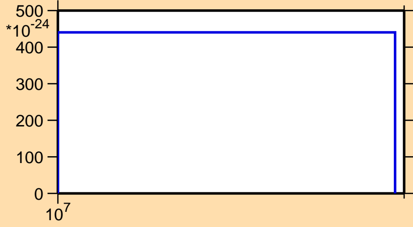
\sigma vs. E for ^{185}\text{Hg} (mt 11)
