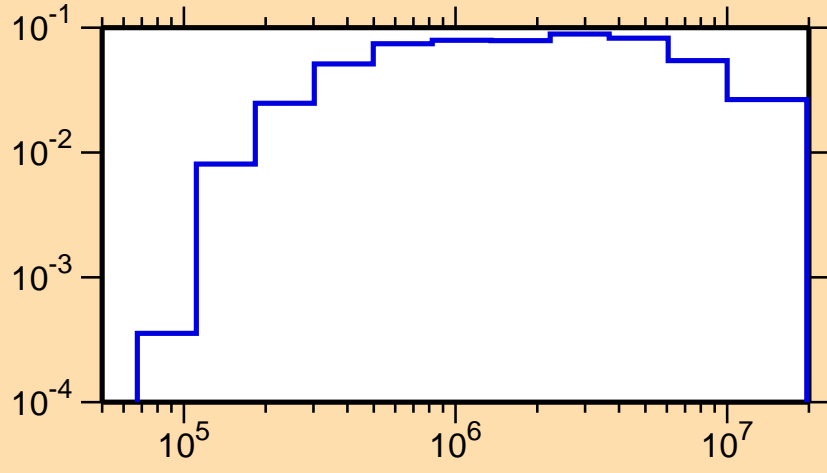
\sigma vs. E for ^{185}\text{Hg}(n,n_3)
