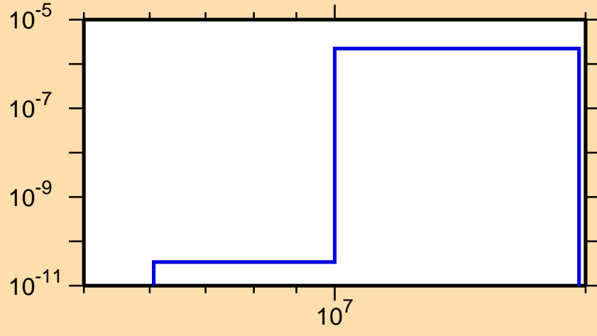
\sigma vs. E for ^{185}\text{Hg}(n,\text{He}3)
