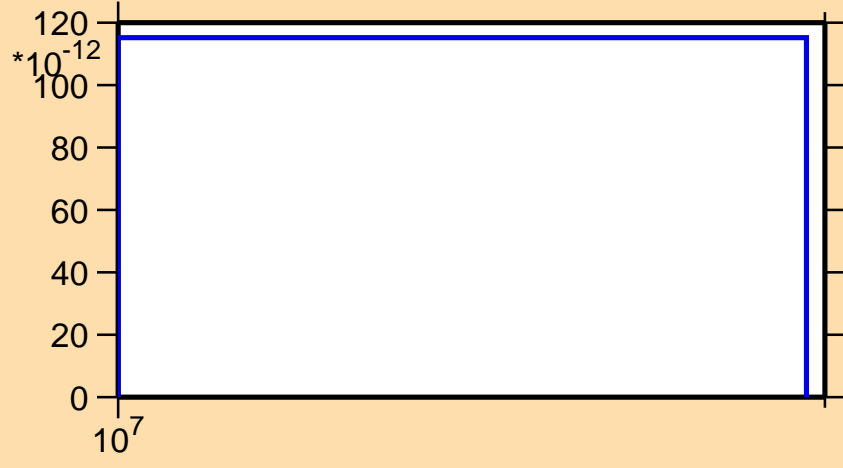
\sigma vs. E for ^{185}\text{Hg}(n,3n\alpha)
