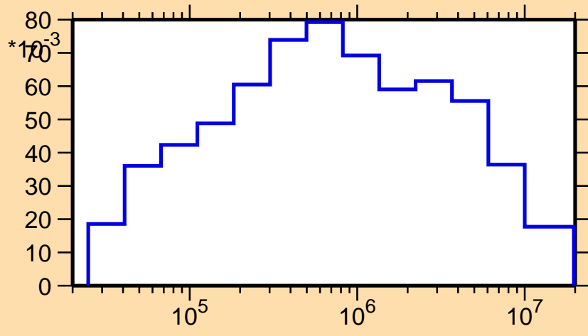
\sigma vs. E for ^{185}\text{Hg}(n,n_1)
