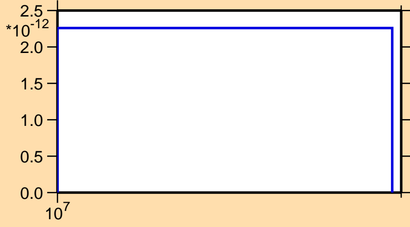
\sigma vs. E for ^{185}\text{Hg}(n,nt)
