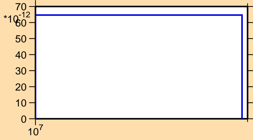
\sigma vs. E for ^{185}\text{Hg} (mt 34)
