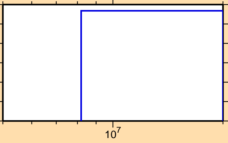
\sigma vs. E for ^{185}\text{Hg}(\text{mt117})
