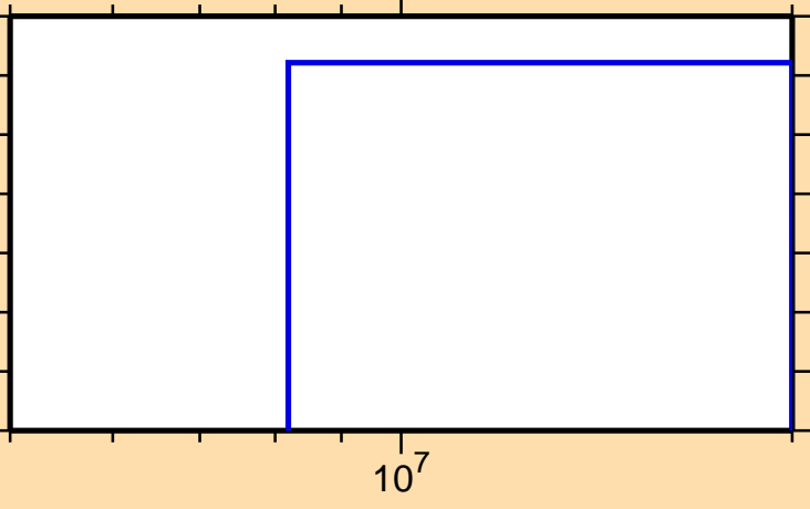
\sigma vs. E for ^{185}\text{Hg}(n,\text{pt})
