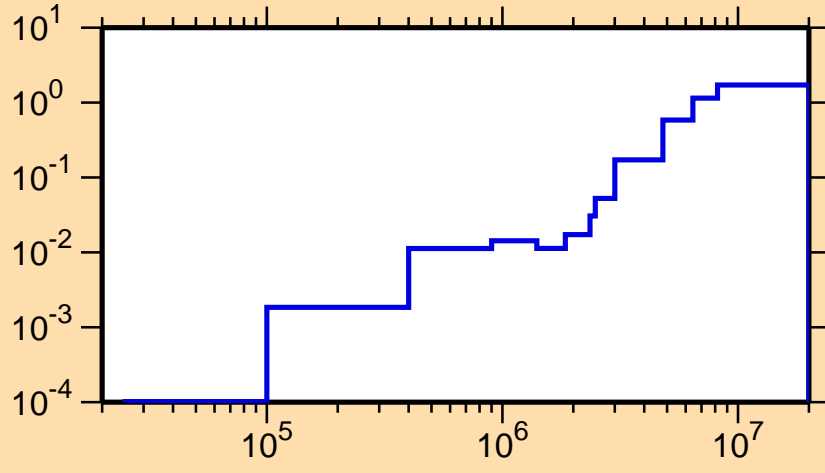
\sigma vs. E for ^{185}\text{Hg}(n,\text{inel.})
