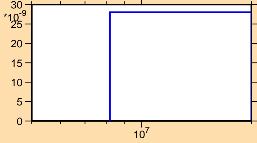
\sigma vs. E for ^{185}\text{Hg} (mt 45)
