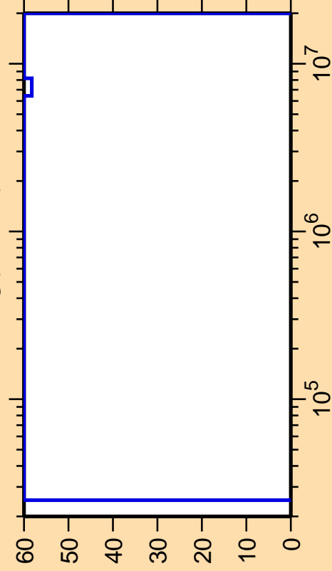
\Delta\sigma/\sigma vs. E for ^{185}\text{Hg}(n,\text{inel.})
