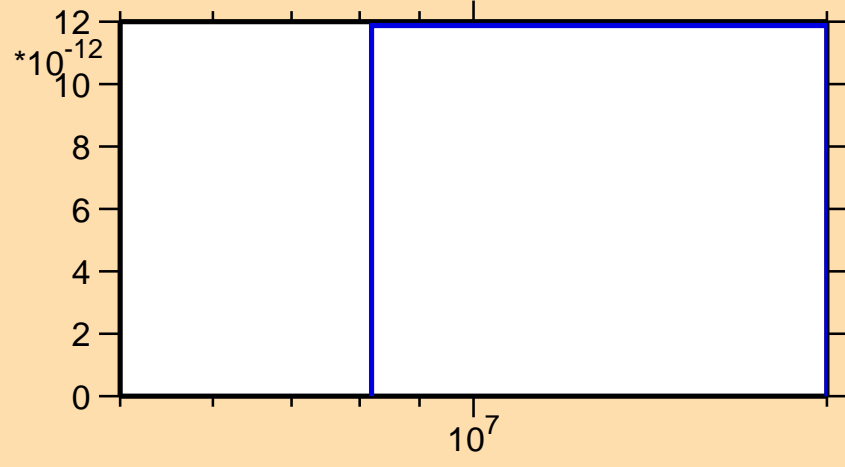
\sigma vs. E for ^{185}\text{Hg}(\text{mt } 34)
