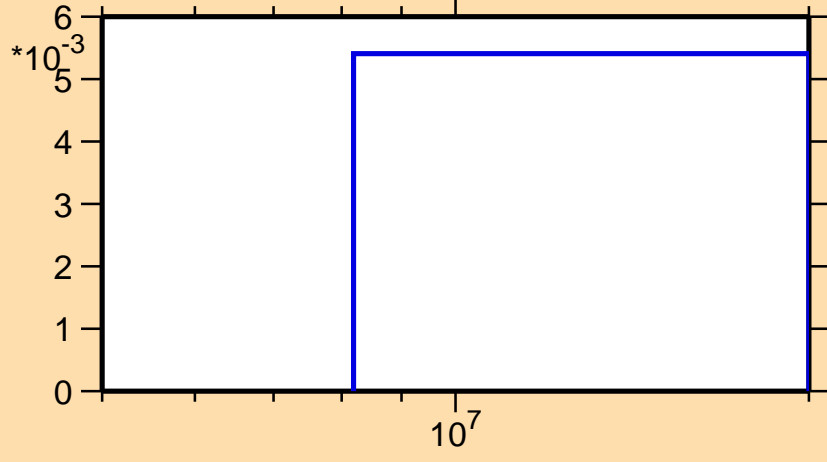
\sigma vs. E for ^{185}\text{Hg}(n,2n\alpha)
