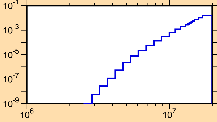
\sigma vs. E for ^{186}\text{Hg}(n,n\alpha)
