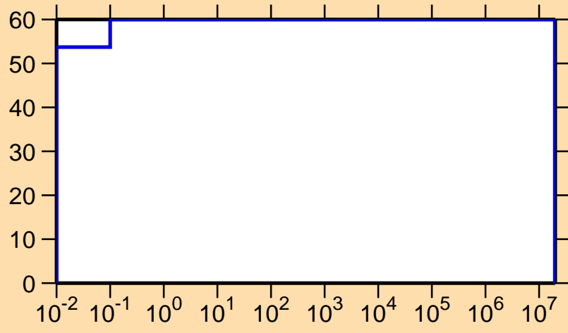
\Delta\sigma/\sigma vs. E for ^{186}\text{Hg}(n,p)
