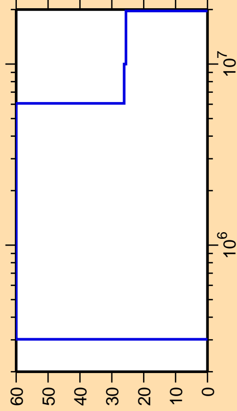
\Delta\sigma/\sigma vs. E for ^{186}\text{Hg}(n,\text{inel.})
