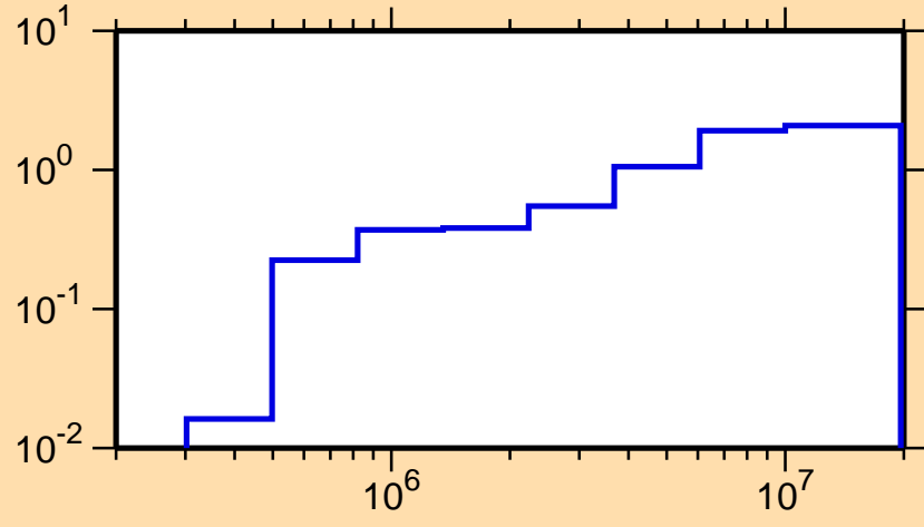
\sigma vs. E for ^{186}\text{Hg}(n,\text{inel.})
