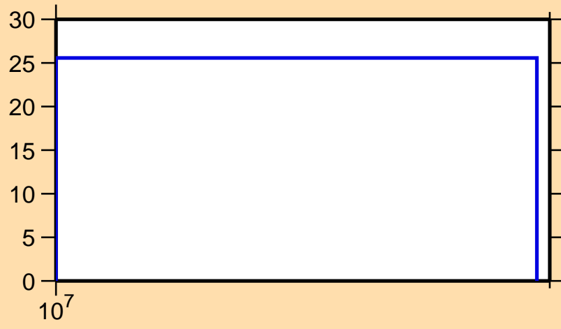
\Delta\sigma/\sigma vs. E for ^{186}\text{Hg}(n,\text{inel.})
