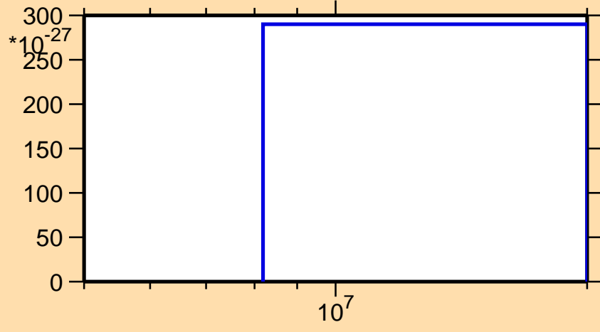
\sigma vs. E for ^{186}\text{Hg} (mt 11)
