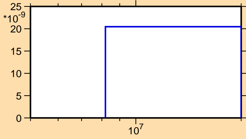
\sigma vs. E for ^{186}\text{Hg} (mt 45)
