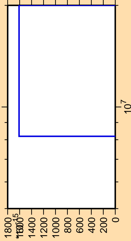
\Delta\sigma/\sigma vs. E for ^{186}\text{Hg} (mt 11)
