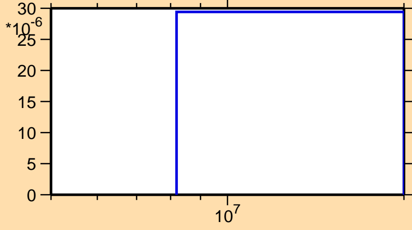
\sigma vs. E for ^{186}\text{Hg}(n,t)
