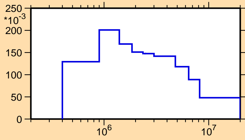
\sigma vs. E for ^{186}\text{Hg}(n,n_1)
