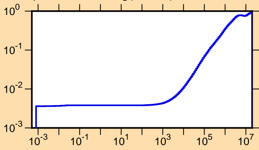
\mu vs. E for ^{187}\text{Hg}(\text{mt251})
