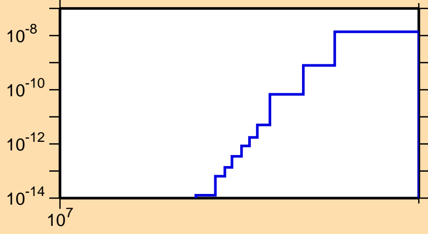
\sigma vs. E for ^{187}\text{Hg}(n,pt)
