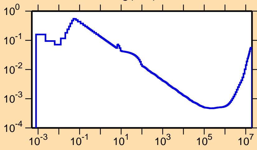
\sigma vs. E for ^{187}\text{Hg}(n,\alpha)
