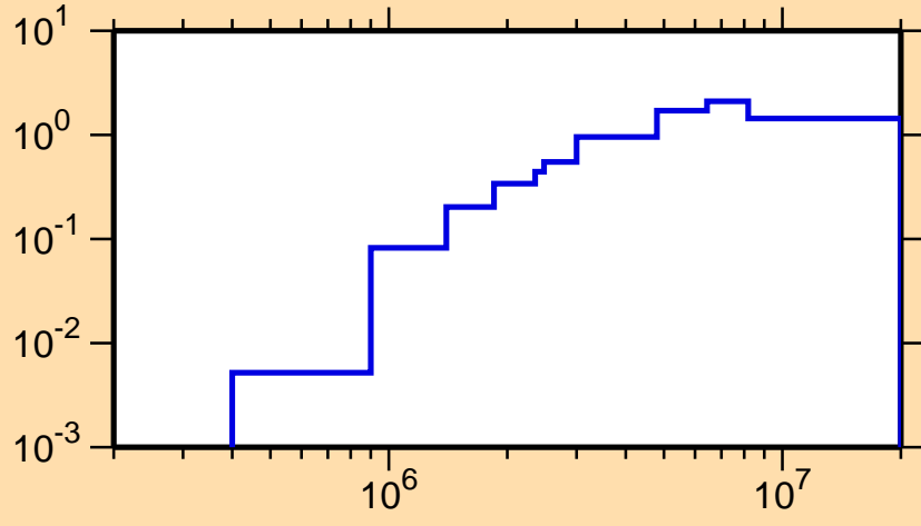
\sigma vs. E for ^{187}\text{Hg}(n,n\text{cont.})
