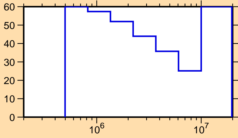
\Delta\sigma/\sigma vs. E for ^{187}\text{Hg}(n,n\text{cont.})
