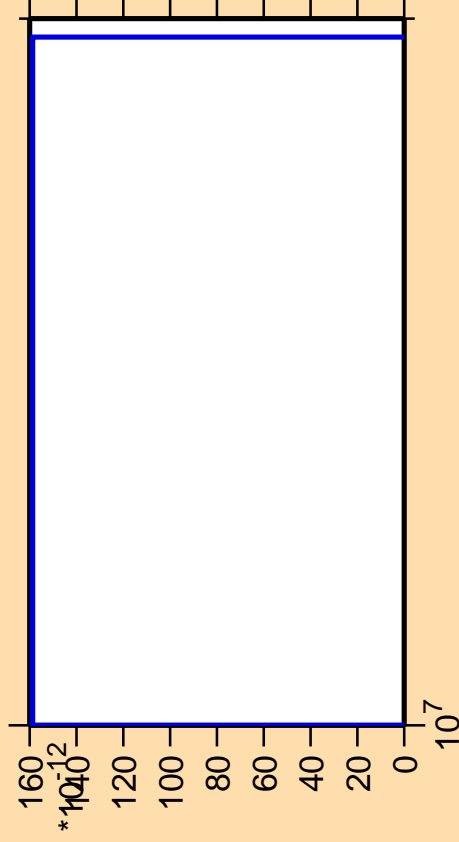
\Delta\sigma/\sigma vs. E for ^{187}\text{Hg} (mt 11)
