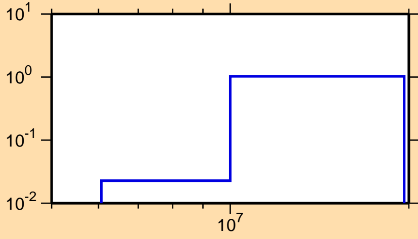
\sigma vs. E for ^{187}\text{Hg}(n,2n)
