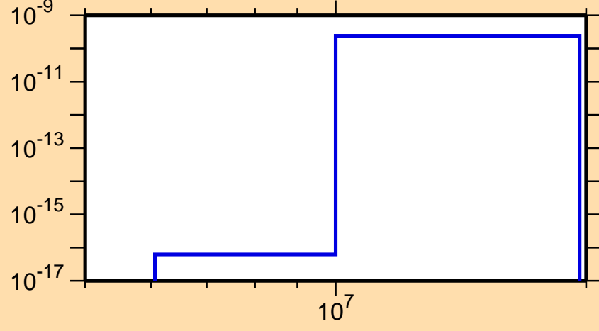
\sigma vs. E for ^{187}\text{Hg}(\text{mt117})
