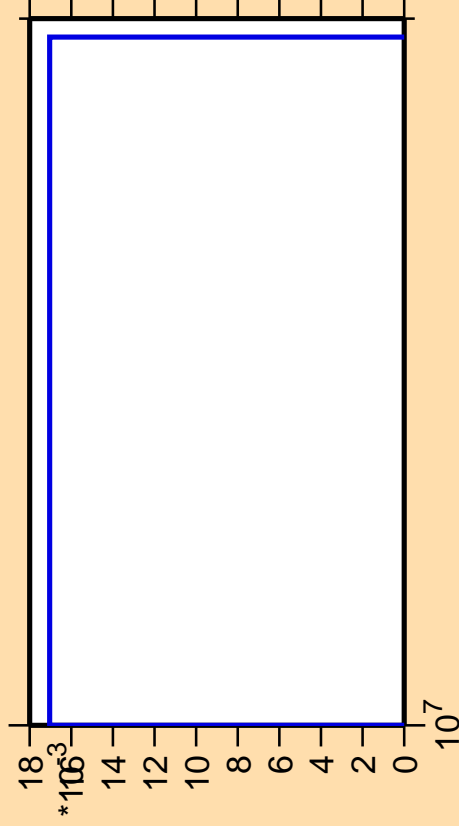
\Delta\sigma/\sigma vs. E for ^{187}\text{Hg}(n,3n\alpha)
