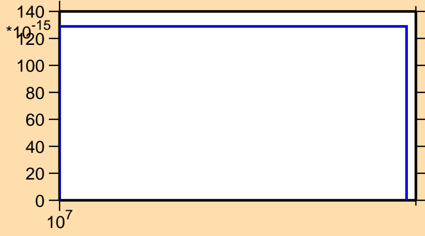
\sigma vs. E for ^{187}\text{Hg}(n,3n\alpha)
