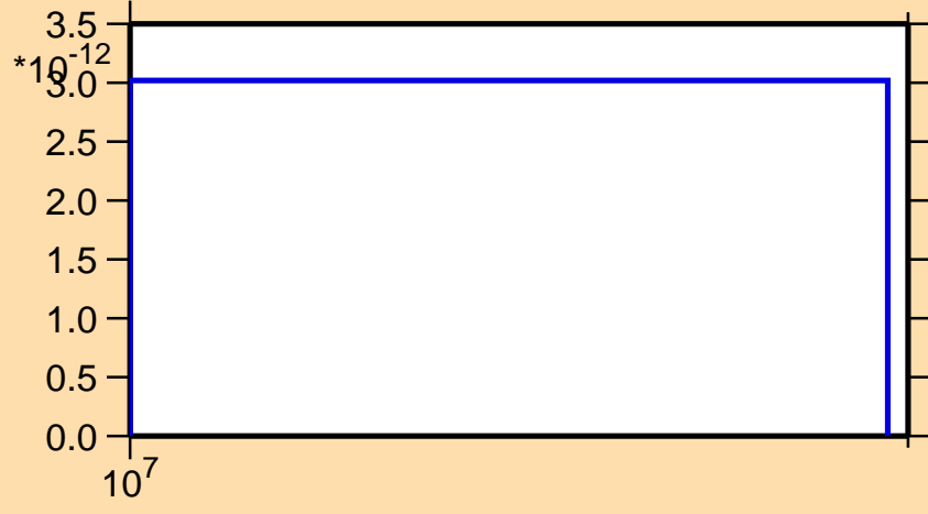
\sigma vs. E for ^{187}\text{Hg}(n,nt)
