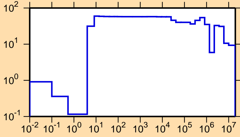
\Delta\sigma/\sigma vs. E for ^{187}\text{Hg}(n,\text{el.})
