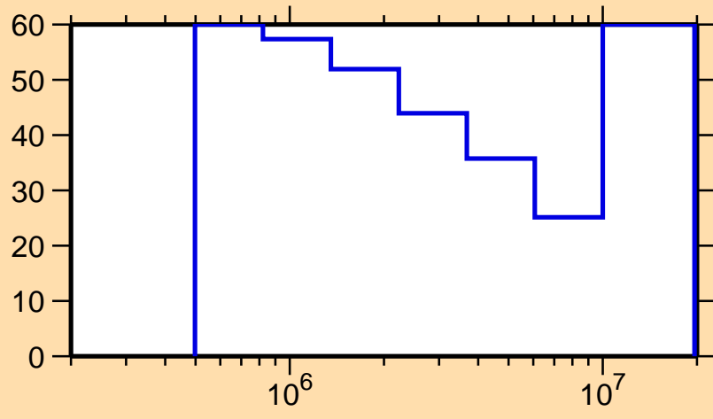
\Delta\sigma/\sigma vs. E for ^{187}\text{Hg}(n,n\text{cont.})
