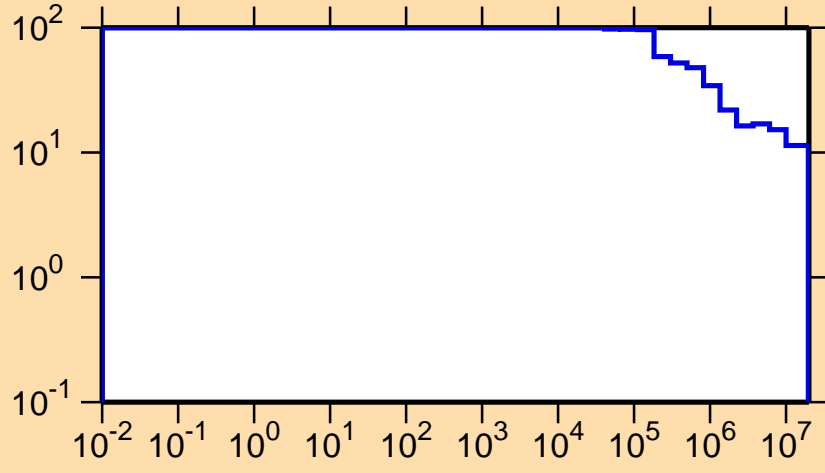
\Delta\sigma/\sigma vs. E for ^{187}\text{Hg}(n,\text{nonel.})
