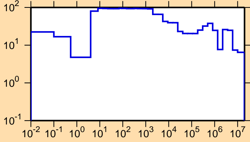
\Delta\sigma/\sigma vs. E for ^{187}\text{Hg}(n,\text{tot.})
