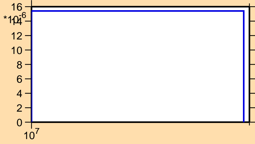
\sigma vs. E for ^{187}\text{Hg}(n,2np)
