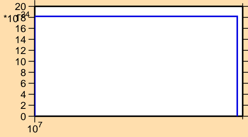
\sigma vs. E for ^{187}\text{Hg} (mt 11)
