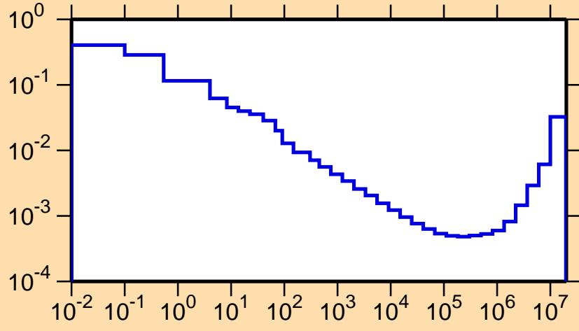
\sigma vs. E for ^{187}\text{Hg}(n,\alpha)
