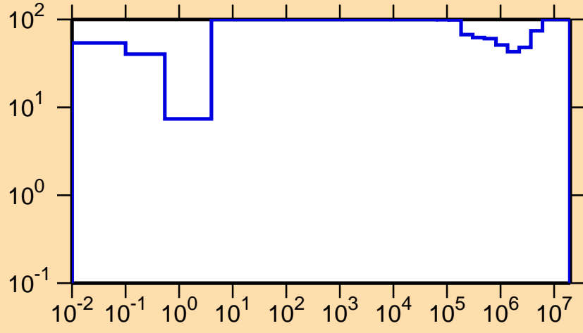
\Delta\sigma/\sigma vs. E for ^{187}\text{Hg}(n,\gamma)
