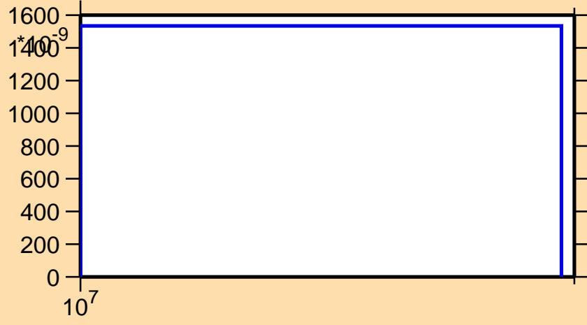
\sigma vs. E for ^{187}\text{Hg}(n,3n)
