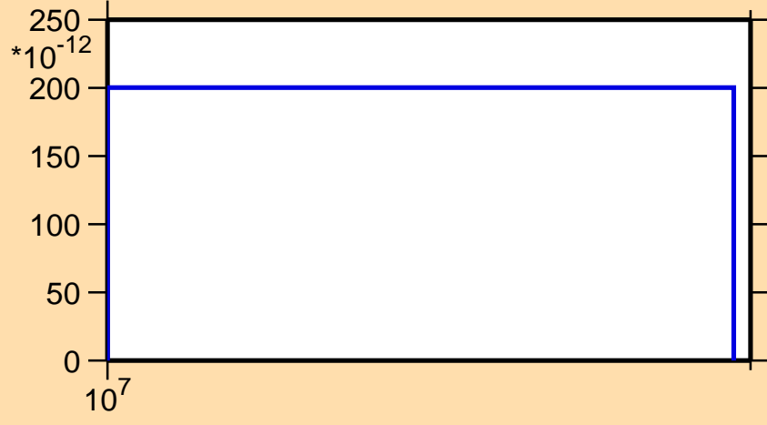
\sigma vs. E for ^{187}\text{Hg}(n,\text{pt})
