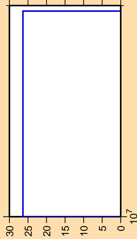
\Delta\sigma/\sigma vs. E for ^{187}\text{Hg}(n,nt)
