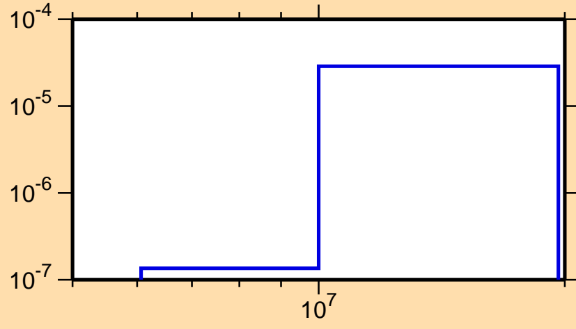
\sigma vs. E for ^{187}\text{Hg}(n,2n\alpha)
