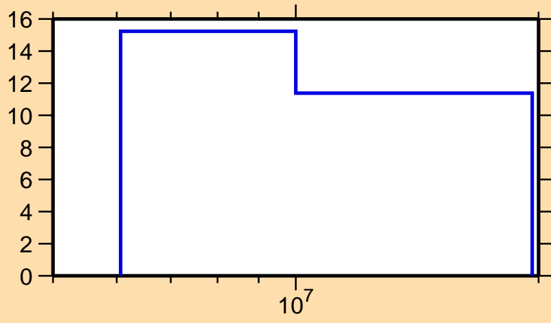
\Delta\sigma/\sigma vs. E for ^{187}\text{Hg}(n,\text{nonel.})
