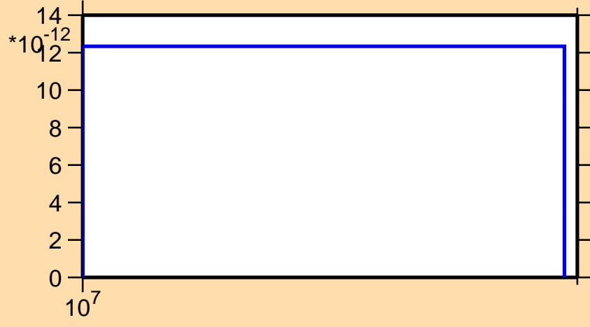
\sigma vs. E for ^{187}\text{Hg} (mt 34)
