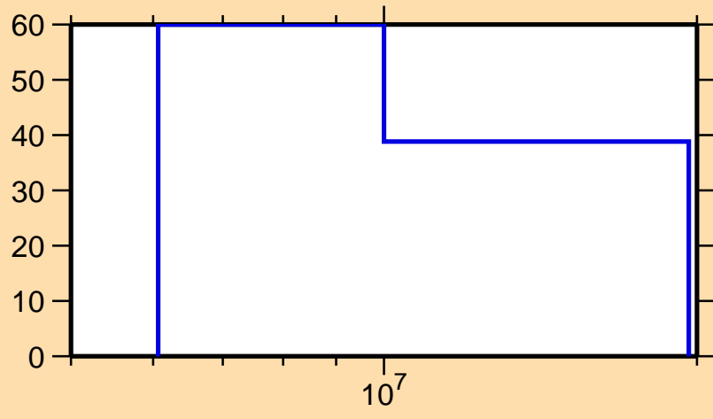
\Delta\sigma/\sigma vs. E for ^{187}\text{Hg}(n,2n)
