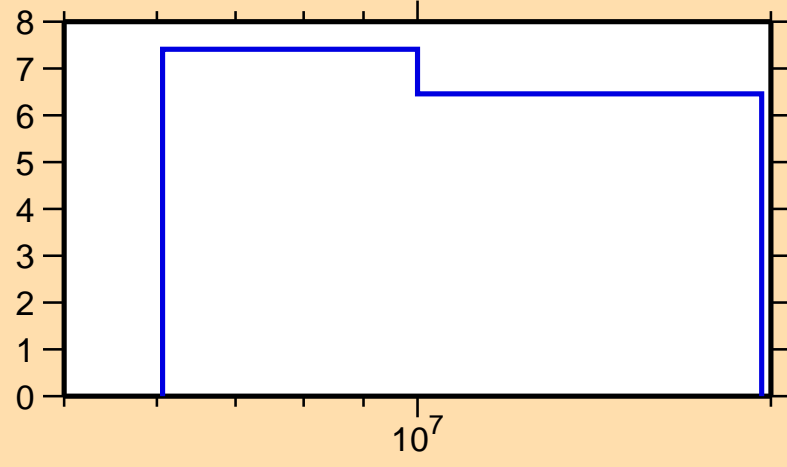
\Delta\sigma/\sigma vs. E for ^{187}\text{Hg}(n,\text{tot.})
