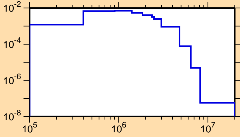
\sigma vs. E for ^{187}\text{Hg}(n,n_3)
