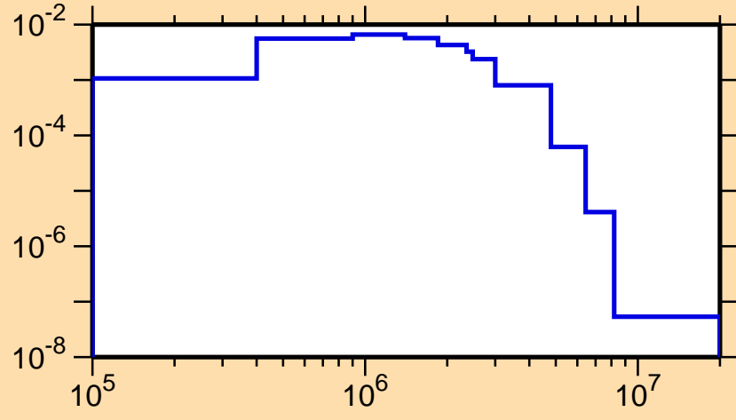
\sigma vs. E for ^{187}\text{Hg}(n,n_2)
