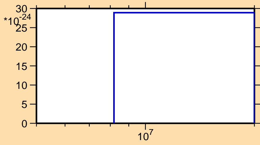
\sigma vs. E for ^{187}\text{Hg} (mt 11)
