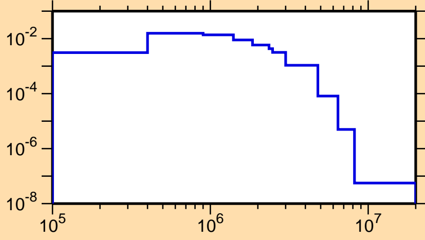
\sigma vs. E for ^{187}\text{Hg}(n,n_4)
