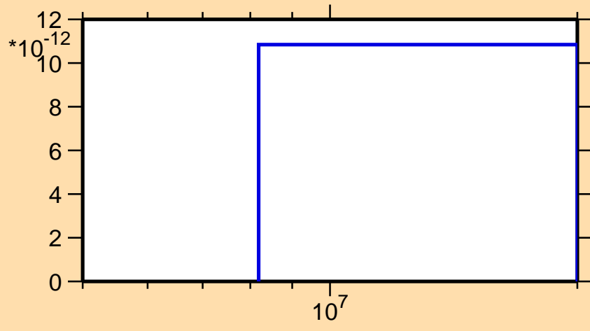
\sigma vs. E for ^{187}\text{Hg}(\text{mt } 34)
