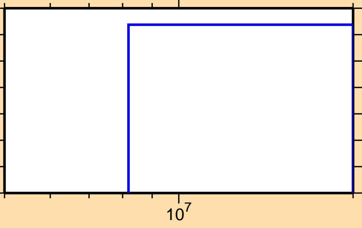
\sigma vs. E for ^{187}\text{Hg}(n,2np)
