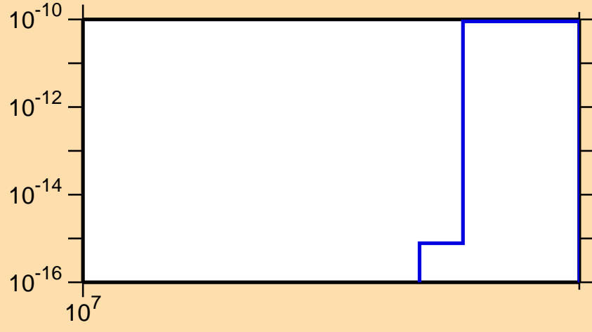
\sigma vs. E for ^{188}\text{Hg}(n,nt)
