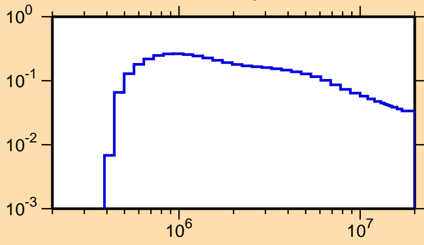
\sigma vs. E for ^{188}\text{Hg}(n,n_1)
