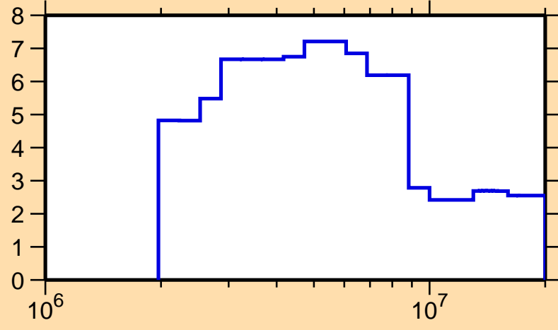
\Delta\sigma/\sigma vs. E for ^{188}\text{Hg}(n,\text{tot.})
