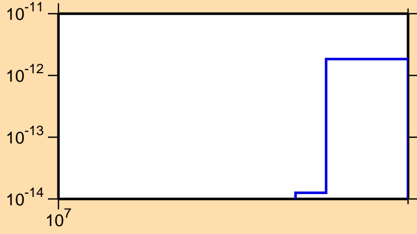
\sigma vs. E for ^{188}\text{Hg} (mt 34)
