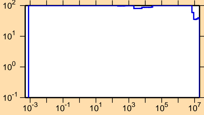
\Delta\sigma/\sigma vs. E for ^{188}\text{Hg}(n,p)
