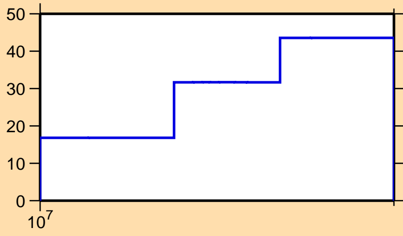
\Delta\sigma/\sigma vs. E for ^{188}\text{Hg}(n,\text{inel.})
