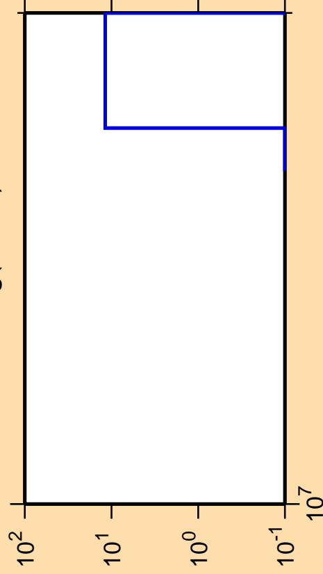
\Delta\sigma/\sigma vs. E for ^{188}\text{Hg} (mt 34)
