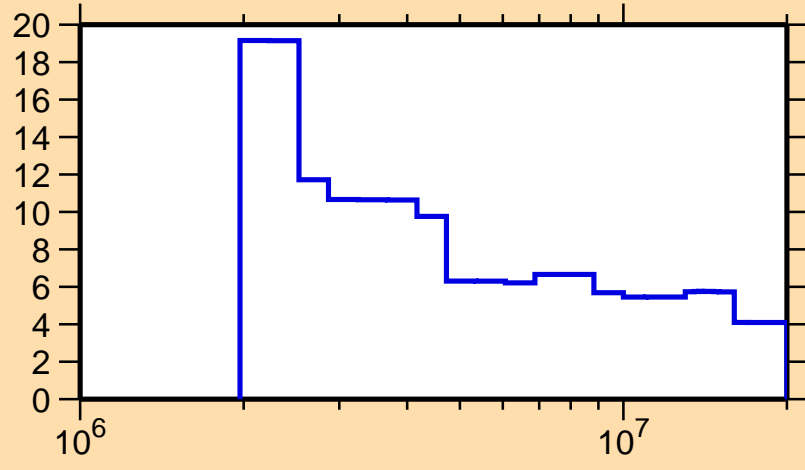
\Delta\sigma/\sigma vs. E for ^{188}\text{Hg}(n,\text{nonel.})
