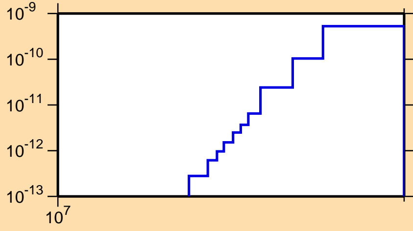
\sigma vs. E for ^{188}\text{Hg}(\text{mt117})
