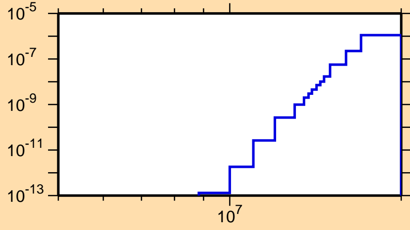
\sigma vs. E for ^{188}\text{Hg}(n,\text{He3})
