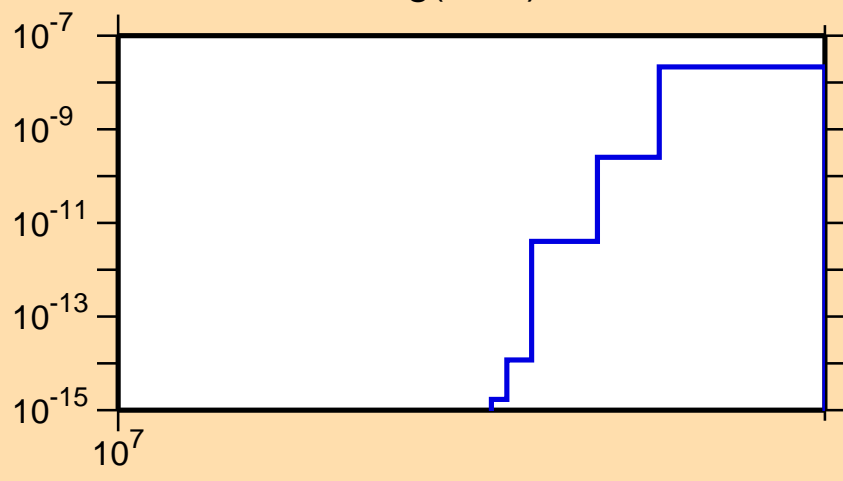
\sigma vs. E for ^{188}\text{Hg}(n,\text{nd})
