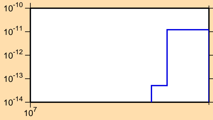
\sigma vs. E for ^{188}\text{Hg}(n,\text{pt})
