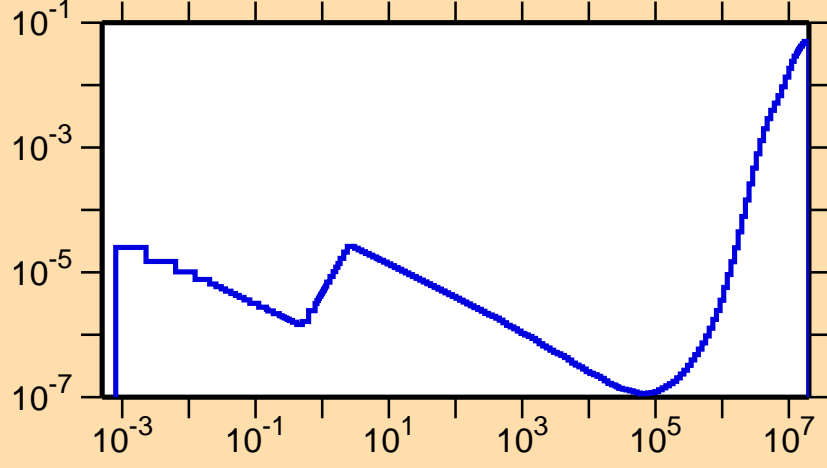
\sigma vs. E for ^{188}\text{Hg}(n,p)
