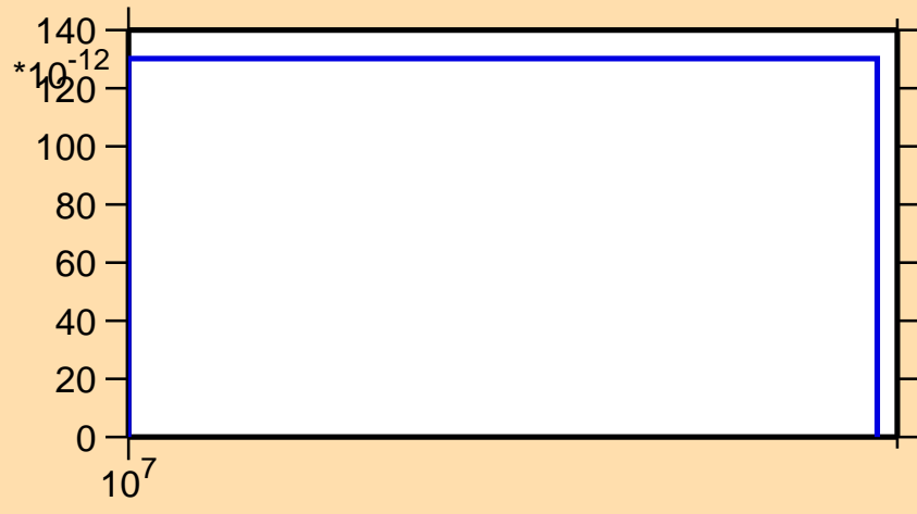
\sigma vs. E for ^{188}\text{Hg}(n,\text{pd})
