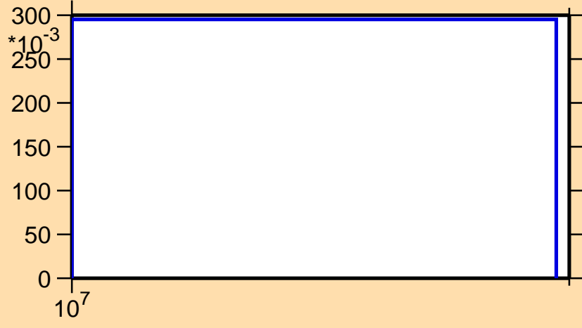
\sigma vs. E for ^{188}\text{Hg}(n,2n)
