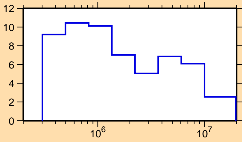
\Delta\sigma/\sigma vs. E for ^{188}\text{Hg}(n,\text{tot.})
