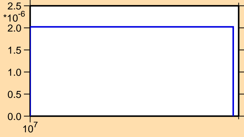
\sigma vs. E for ^{188}\text{Hg}(n,3n)
