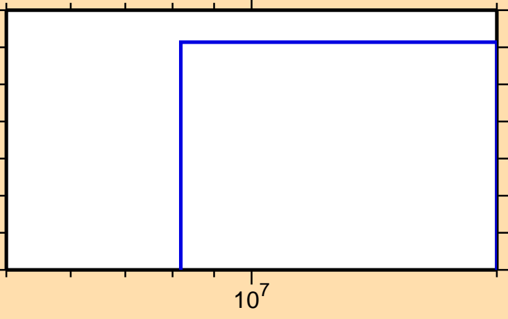
\sigma vs. E for ^{188}\text{Hg}(\text{mt117})
