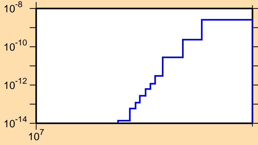
\sigma vs. E for ^{189}\text{Hg}(n,\text{pd})
