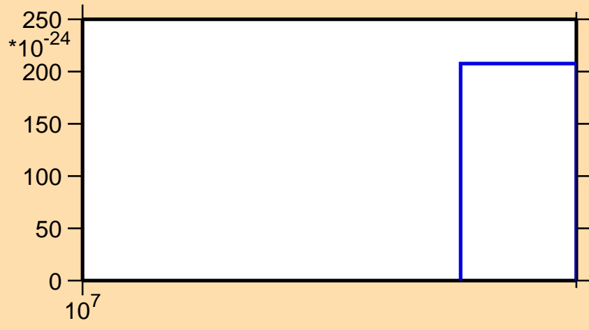
\sigma vs. E for ^{189}\text{Hg} (mt 11)
