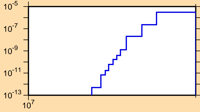
\sigma vs. E for ^{189}\text{Hg}(n,\text{nd})
