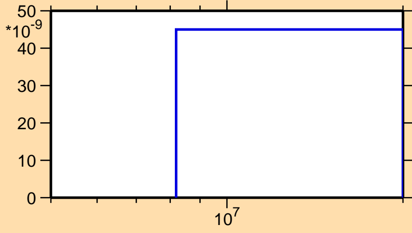
\sigma vs. E for ^{189}\text{Hg}(n,\text{He}3)
