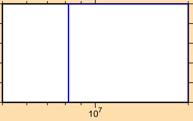
\sigma vs. E for ^{189}\text{Hg}(n,3n)
