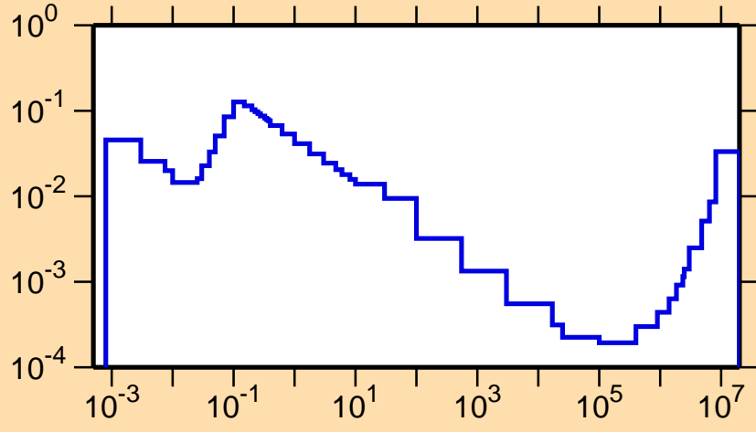
\sigma vs. E for ^{189}\text{Hg}(n,p)
