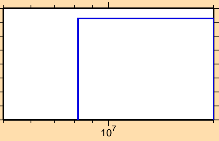
\sigma vs. E for ^{189}\text{Hg}(n,\text{nd})
